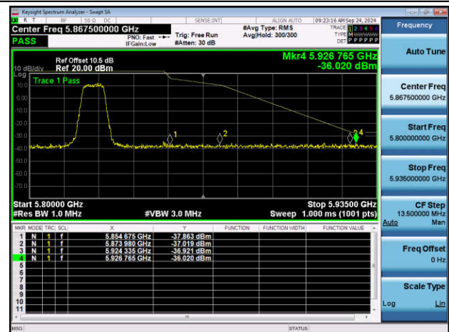
11A(10MHZ)-Ant1-5825-PASS
