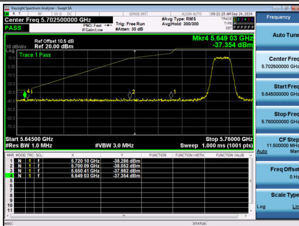
11A(10MHZ)-Ant1-5745-PASS
