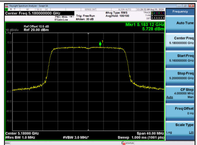
11AX20SISO-Ant2-5180-PASS
