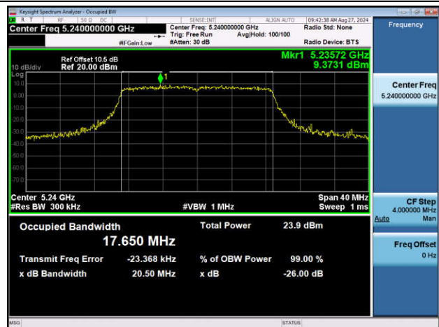
11N20SISO-Ant2-5240
