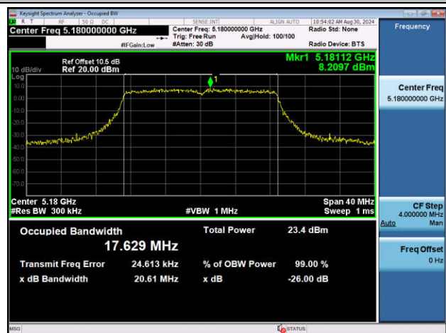
11AC20SISO-Ant2-5180
