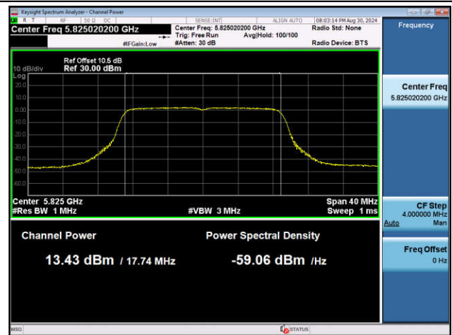
11N20SISO-Ant1-5825-PASS
