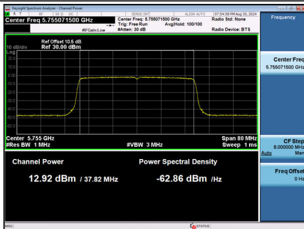
11AX40SISO-Ant2-5755-PASS
