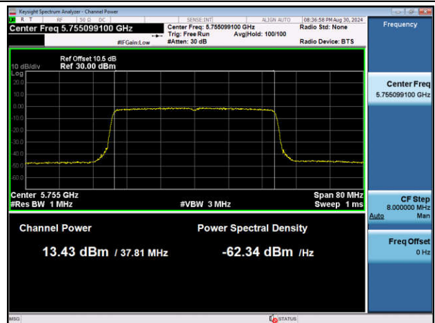
11AX40SISO-Ant1-5755-PASS
