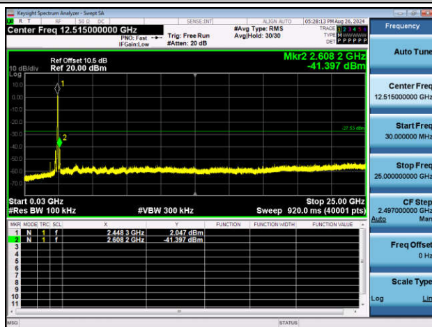
11N40SISO-Ant1-2452-30~25000-PASS
