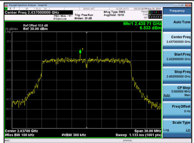
11N20SISO-Ant2-2437-0~Reference-PASS
