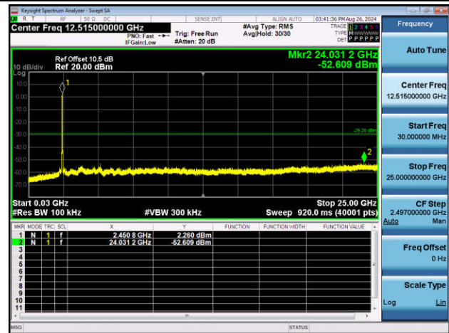
11N40SISO-Ant2-2452-0~Reference-PASS
