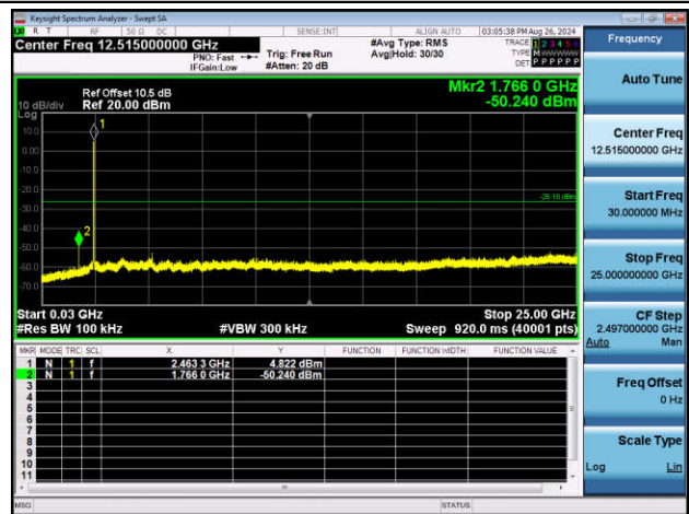
11G-Ant2-2462-30~25000-PASS
