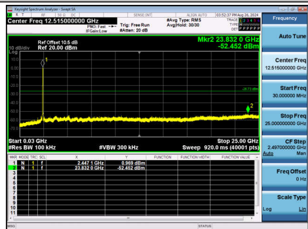
11N40SISO-Ant2-2452-30~25000-PASS
