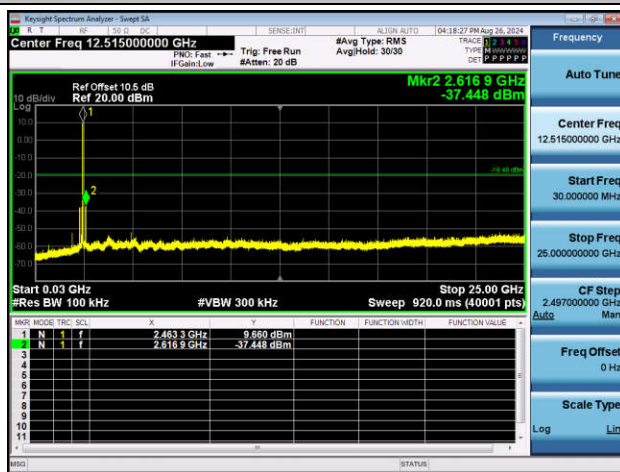
11B-Ant1-2462-30~25000-PASS
