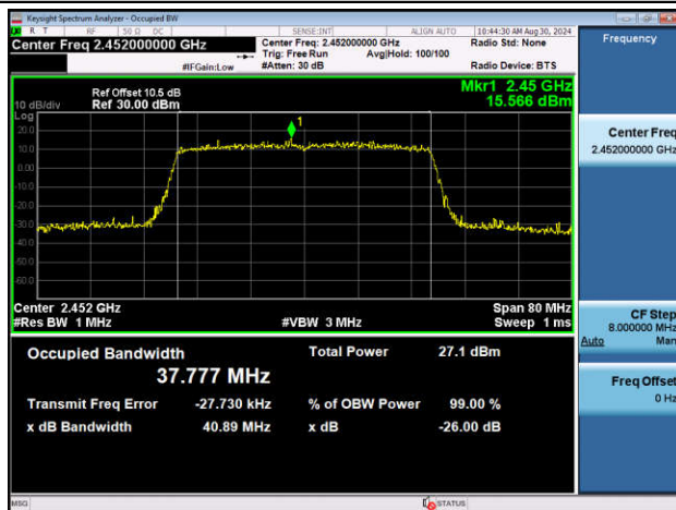
11AX40SISO-Ant2-2452
