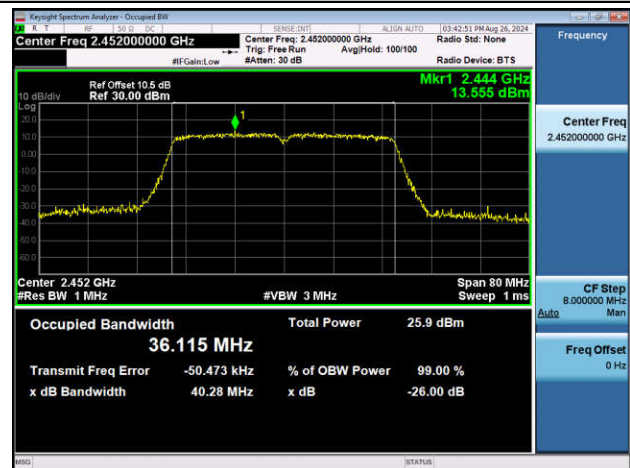
11N40SISO-Ant2-2452
