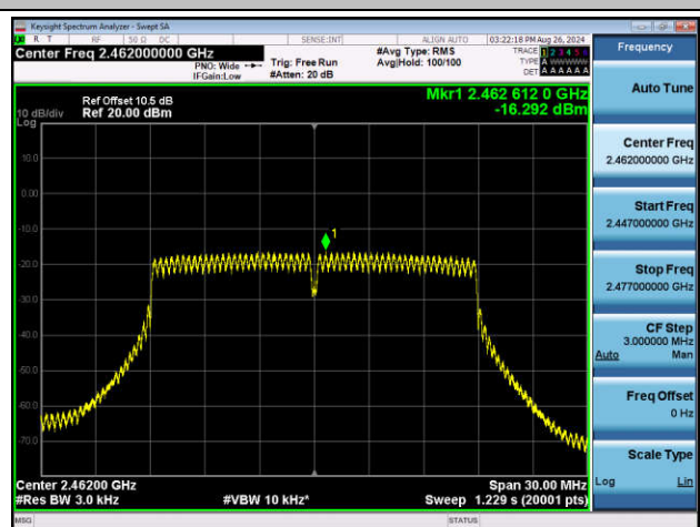
11N20SISO-Ant2-2462-PASS
