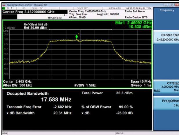
11N20SISO-Ant1-2462
