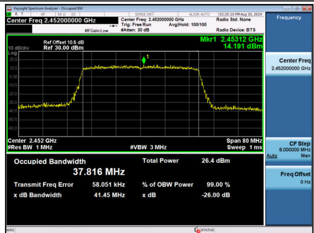
11AX40SISO-Ant1-2452
