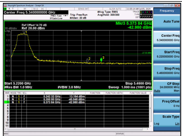
11AC20SISO-Ant1-5240-PASS
