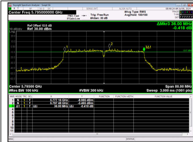
11AC40SISO-Ant1-5795-PASS
