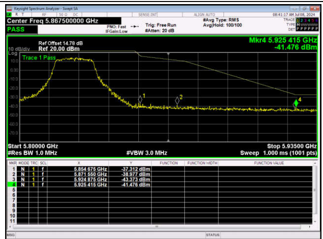
11AC20SISO-Ant1-5825-PASS
