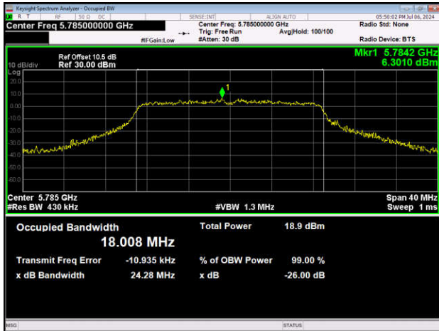
11N20SISO-Ant1-5785
