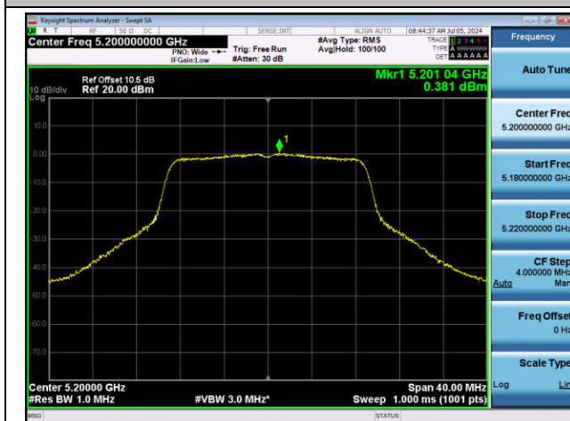
11N20SISO-Ant1-5200-PASS
