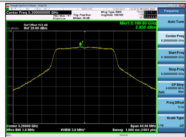
11A-Ant1-5200-PASS
