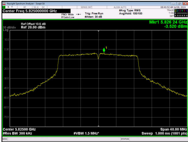
11AC20SISO-Ant1-5825-PASS
