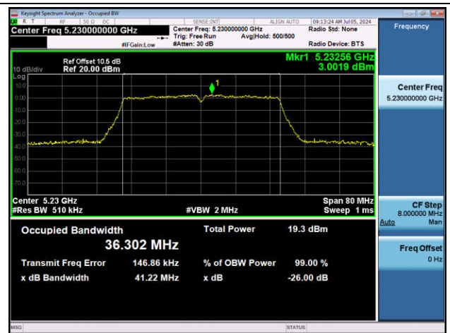
11N40SISO-Ant1-5230
