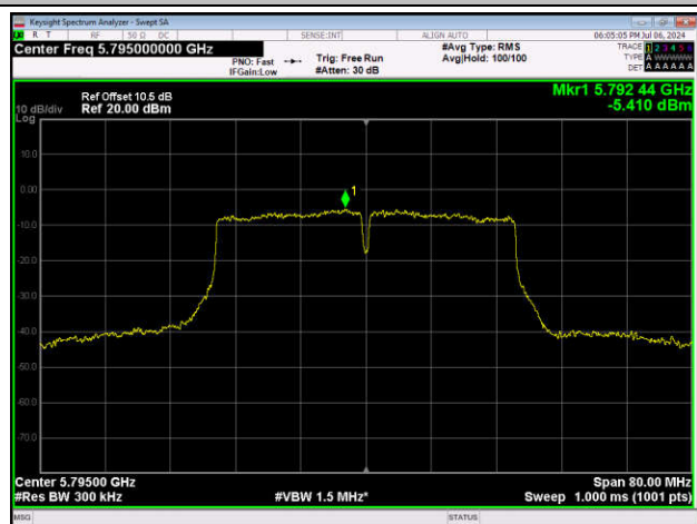
11N40SISO-Ant1-5795-PASS
