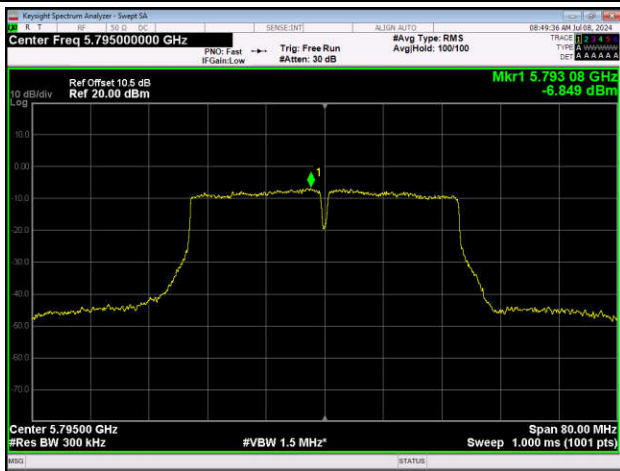
11AC40SISO-Ant1-5795-PASS
