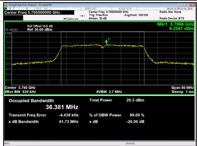
11N40SISO-Ant1-5795
