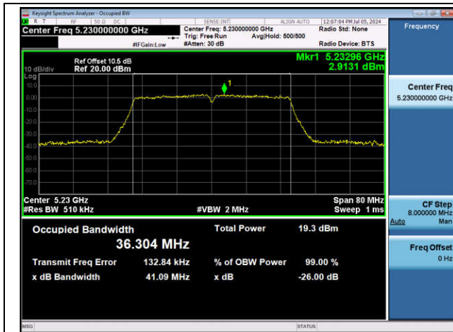
11AC40SISO-Ant1-5230
