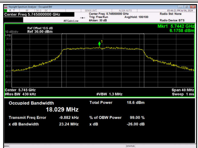
11N20SISO-Ant1-5745
