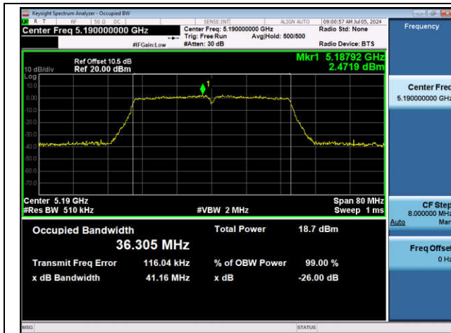
11N40SISO-Ant1-5190
