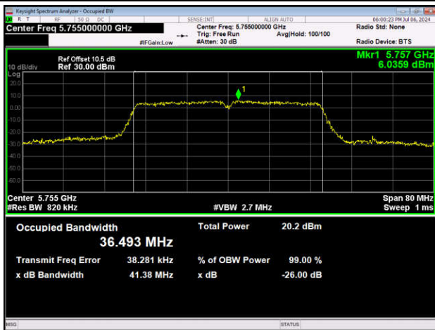
11N40SISO-Ant1-5755
