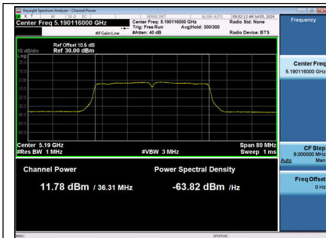
11N40SISO-Ant1-5190-PASS
