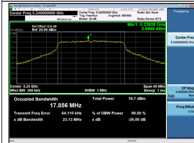
11AC20SISO-Ant1-5240
