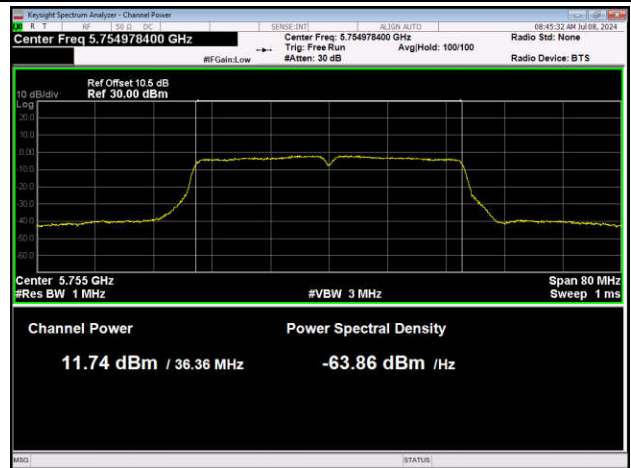
11AC40SISO-Ant1-5755-PASS
