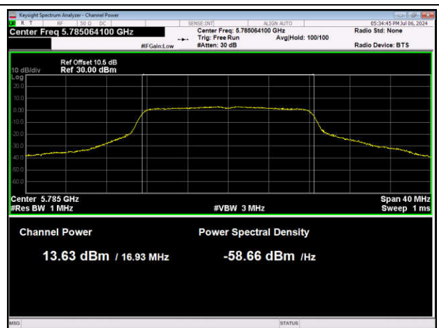
11A-Ant1-5785-PASS
