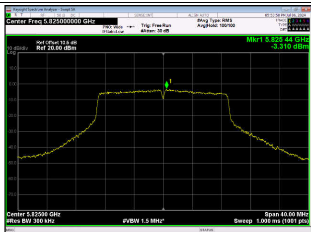
11N20SISO-Ant1-5825-PASS
