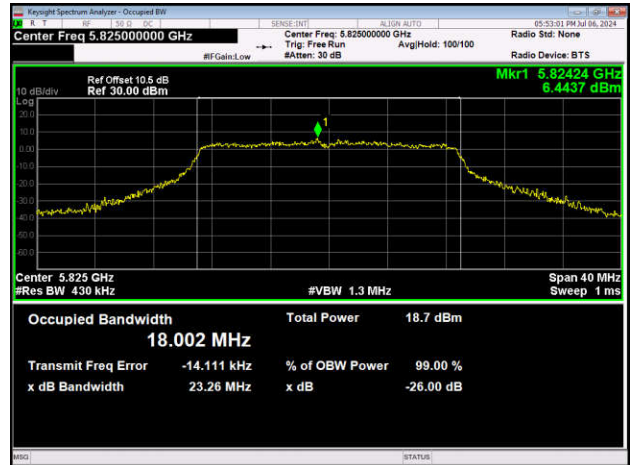
11N20SISO-Ant1-5825
