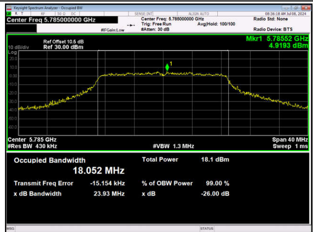
11AC20SISO-Ant1-5785
