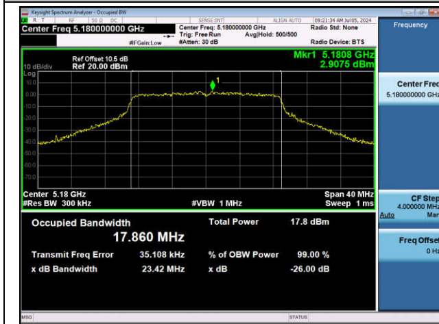
11AC20SISO-Ant1-5180
