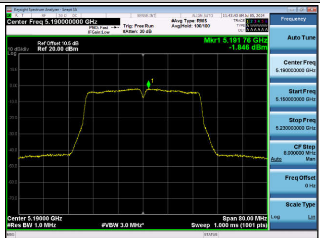
11AC40SISO-Ant1-5190-PASS
