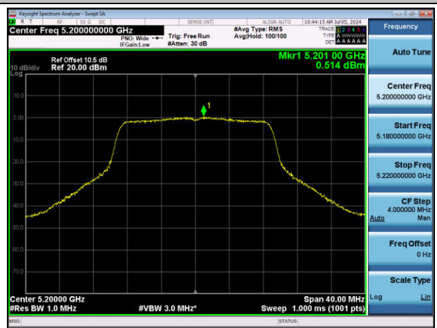
11AC20SISO-Ant1-5200-PASS
