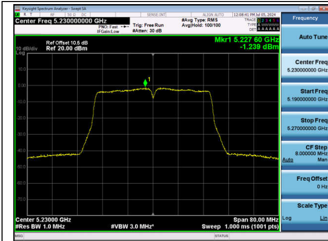
11AC40SISO-Ant1-5230-PASS
