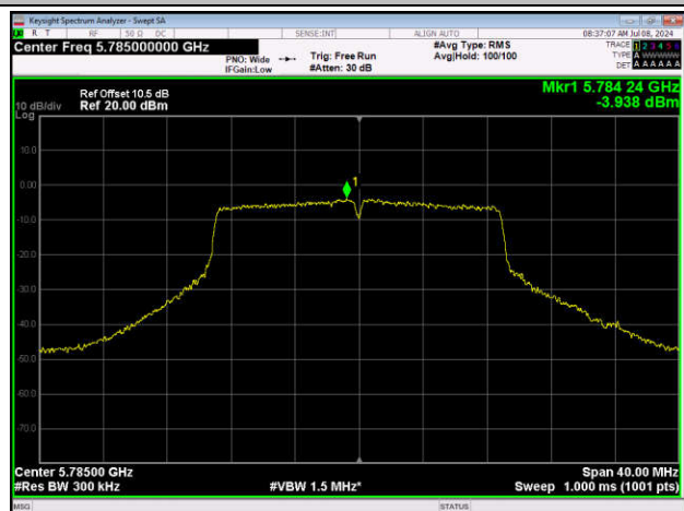
11AC20SISO-Ant1-5785-PASS
