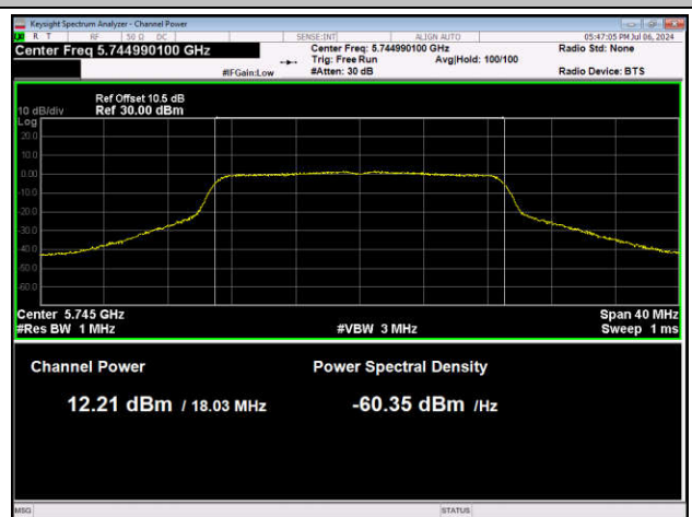
11N20SISO-Ant1-5745-PASS
