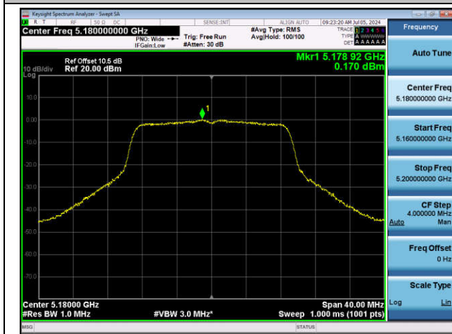
11AC20SISO-Ant1-5180-PASS
