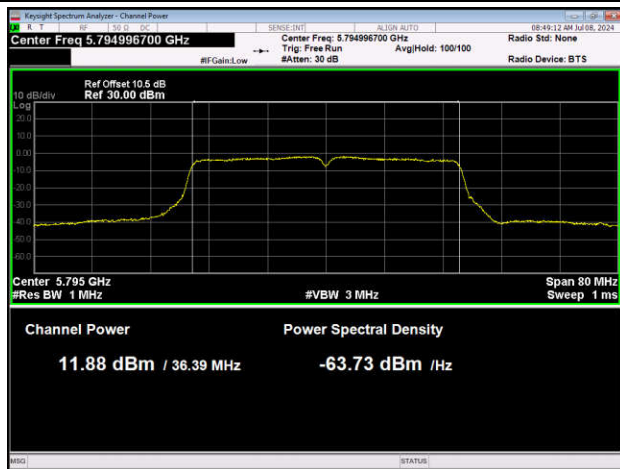
11AC40SISO-Ant1-5795-PASS
