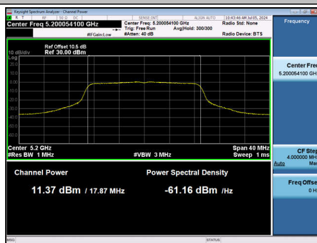
11AC20SISO-Ant1-5200-PASS
