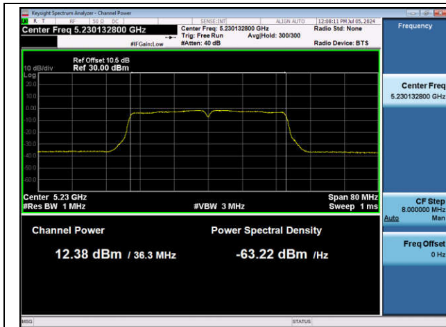
11AC40SISO-Ant1-5230-PASS
