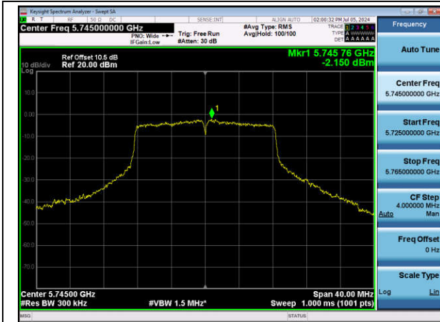
11A-Ant1-5745-PASS
