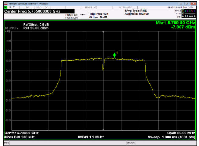
11AC40SISO-Ant1-5755-PASS
