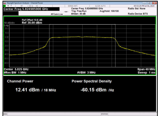
11N20SISO-Ant1-5825-PASS
