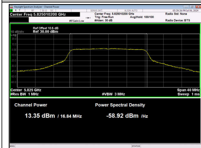
11A-Ant1-5825-PASS
