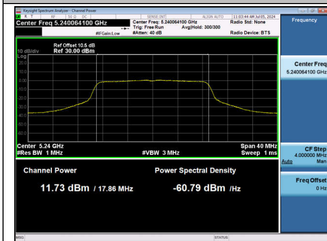
11AC20SISO-Ant1-5240-PASS
