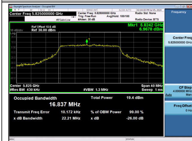
11A-Ant1-5825
