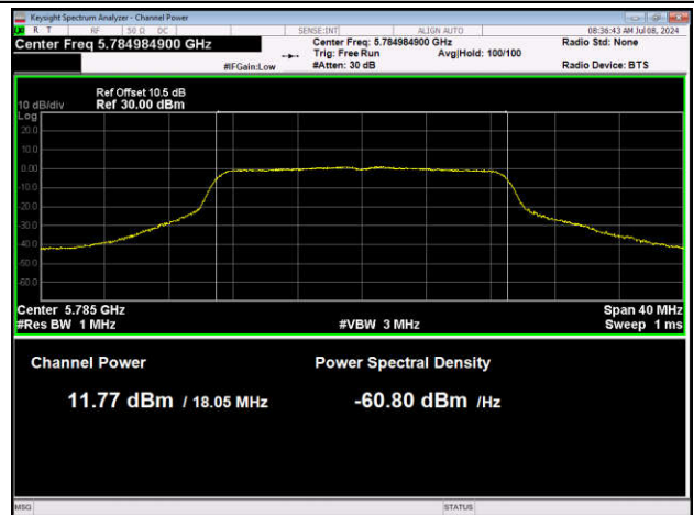
11AC20SISO-Ant1-5785-PASS
