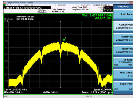
11B-Ant1-2437-PASS
