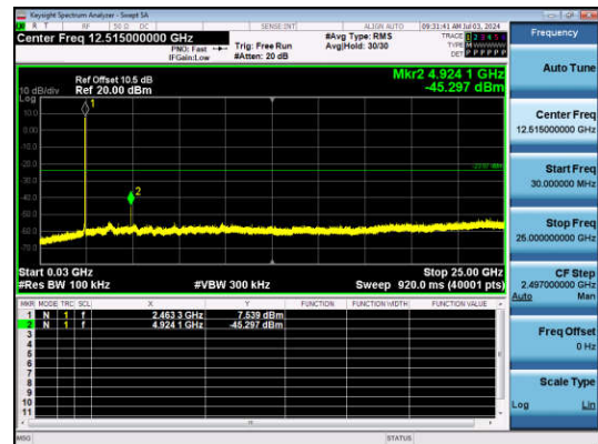
11B-Ant1-2462-30~25000-PASS
