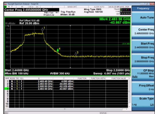
11N20SISO-Ant1-2462-PASS
