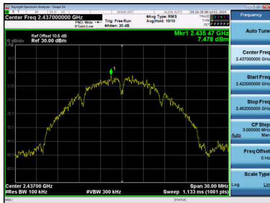
11B-Ant1-2437-0~Reference-PASS
