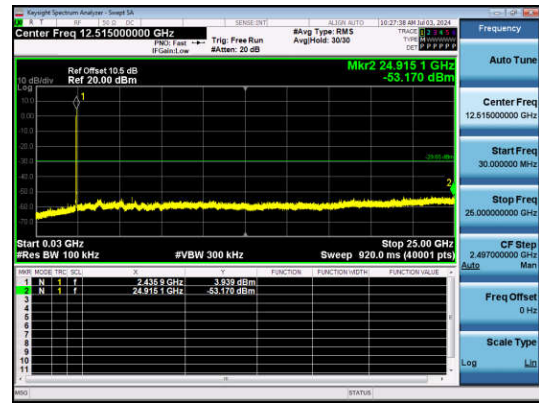
11N20SISO-Ant1-2437-30~25000-PASS
