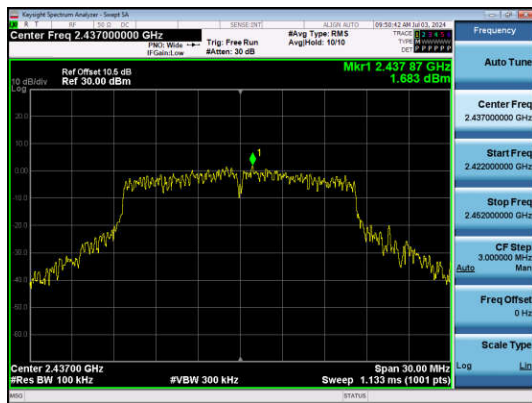
11G-Ant1-2437-0~Reference-PASS
