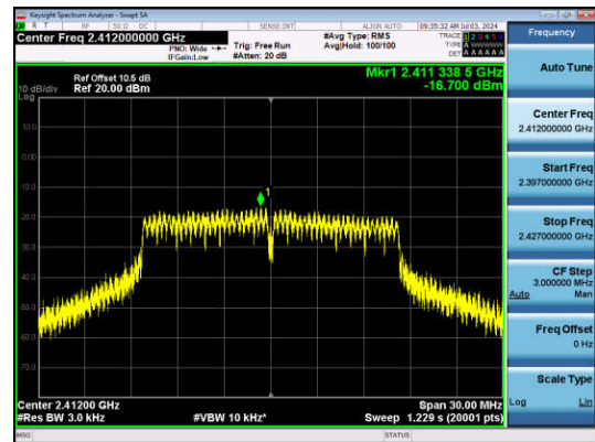
11G-Ant1-2412-PASS
