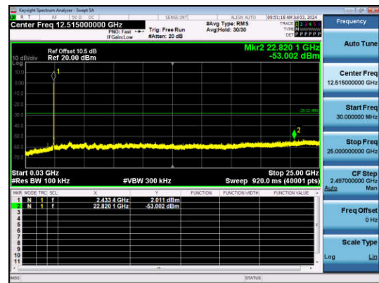
11G-Ant1-2437-30~25000-PASS
