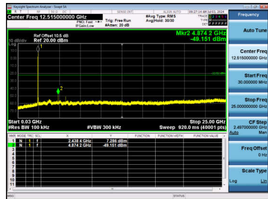
11B-Ant1-2437-30~25000-PASS
