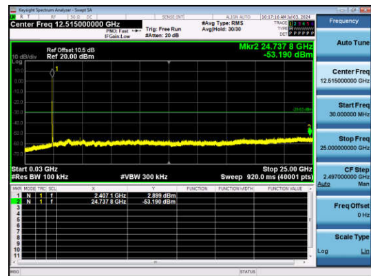
11N20SISO-Ant1-2412-30~25000-PASS
