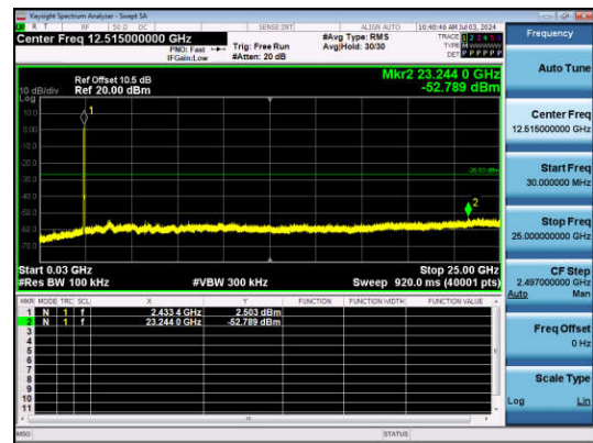
11N40SISO-Ant1-2422-30~25000-PASS
