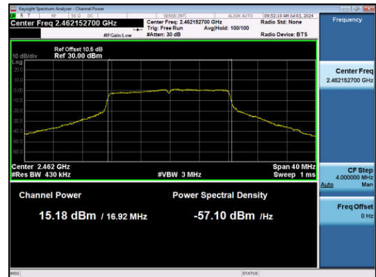
11G-Ant1-2462-PASS
