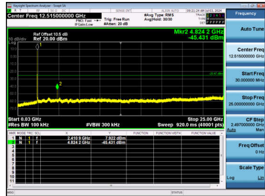
11B-Ant1-2412-30~25000-PASS
