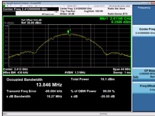
11B-Ant1-2412
