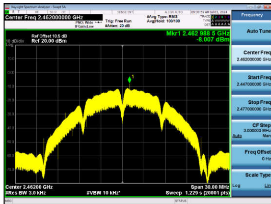
11B-Ant1-2462-PASS
