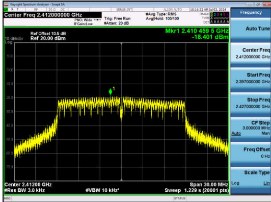
11N20SISO-Ant1-2412-PASS
