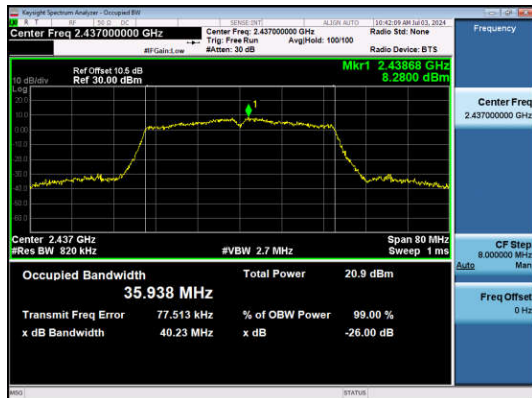
11N40SISO-Ant1-2437
