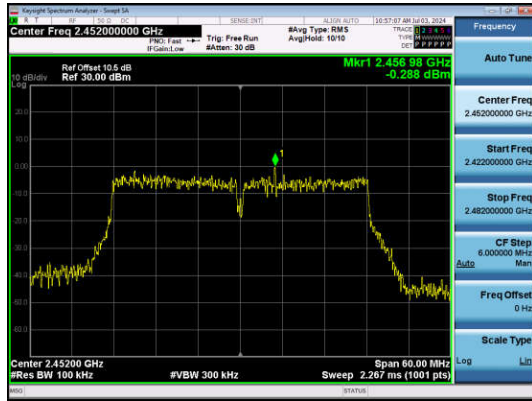
11N40SISO-Ant1-2452-0~Reference-PASS
