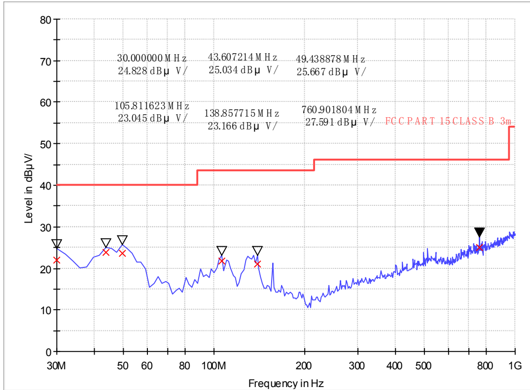
EMI Sweep-3M(30-1G)
