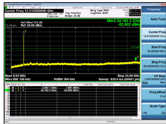
11N20SISO-Ant1-2462-30~25000-PASS
