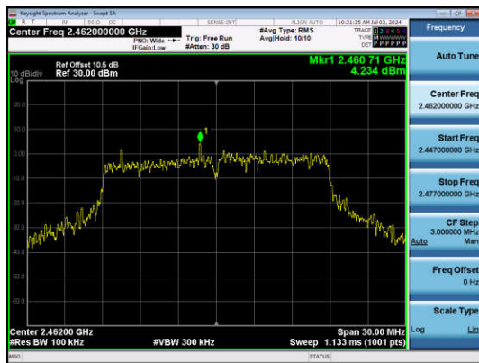
11N20SISO-Ant1-2462-0~Reference-PASS
