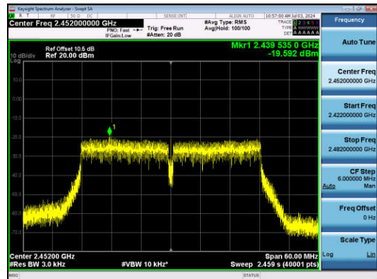
11N40SISO-Ant1-2452-PASS
