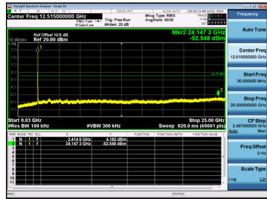
11G-Ant1-2412-30~25000-PASS
