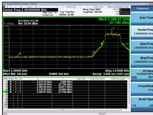
11G-Ant1-2412-PASS
