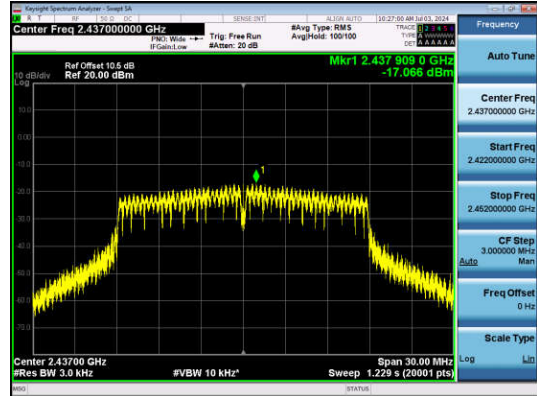
11N20SISO-Ant1-2437-PASS
