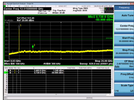
11G-Ant1-2462-30~25000-PASS
