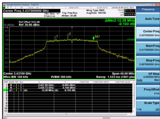
11G-Ant1-2437-PASS
