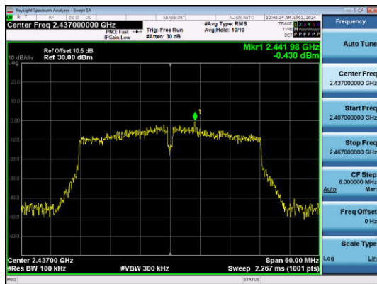
11N40SISO-Ant1-2437-0~Reference-PASS
