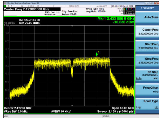
11N40SISO-Ant1-2422-PASS
