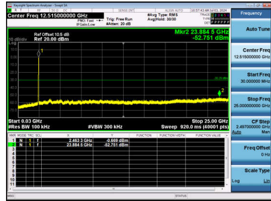
11N40SISO-Ant1-2452-30~25000-PASS
