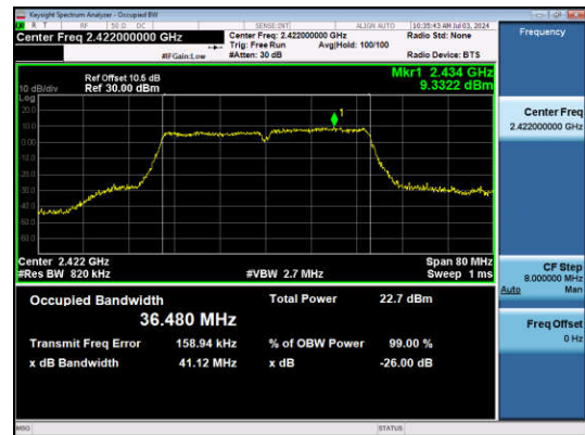
11N40SISO-Ant1-2422
