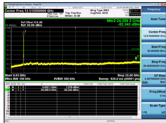
11N40SISO-Ant1-2437-30~25000-PASS
