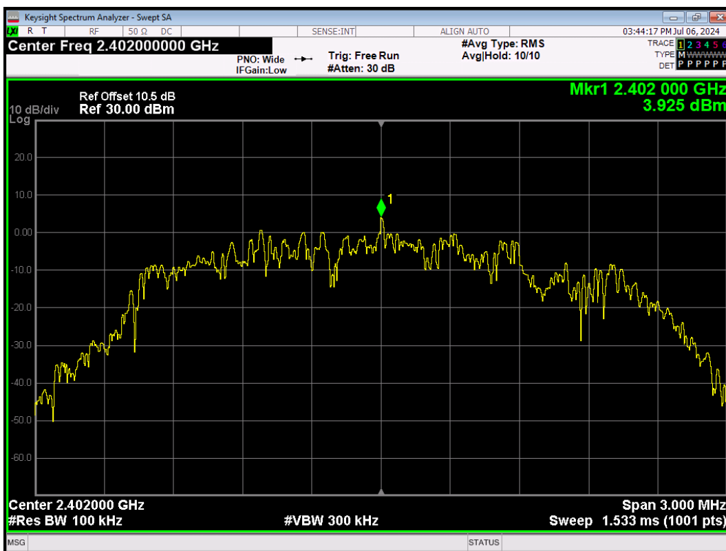
BLE_2M-Ant1-2402-0~Reference-PASS
