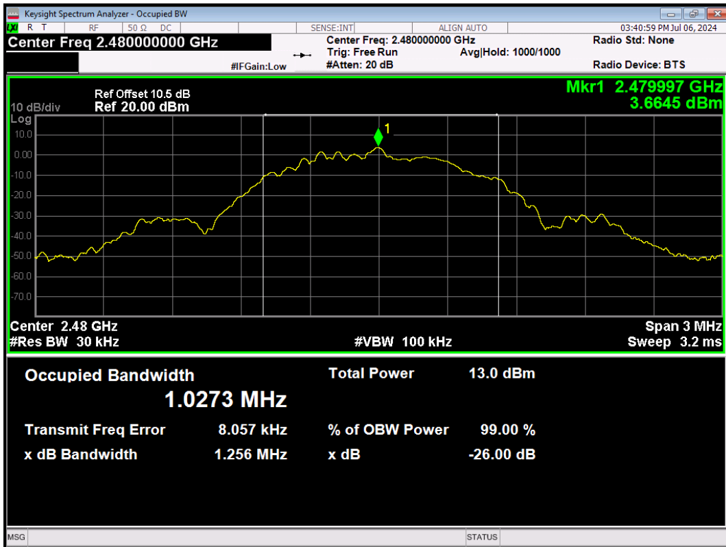
BLE_1M-Ant1-2480
