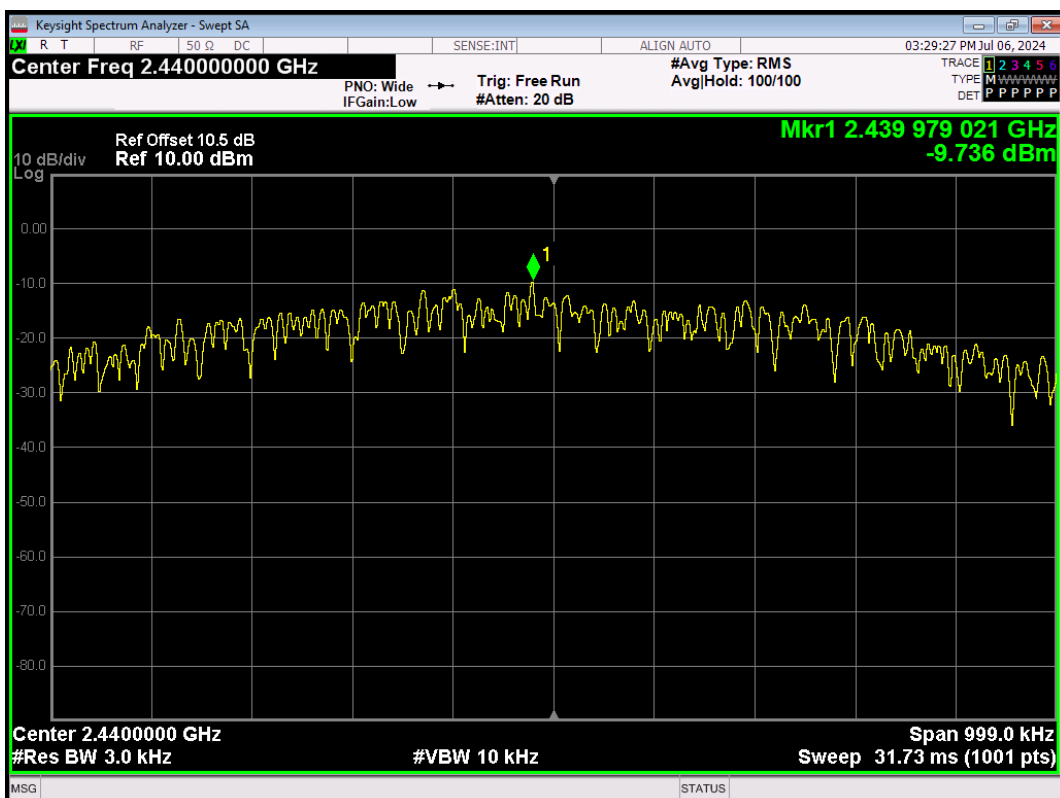
BLE_1M-Ant1-2440-PASS
