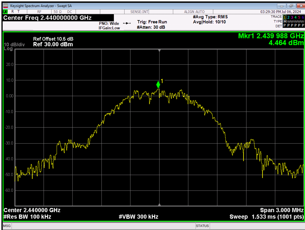
BLE_1M-Ant1-2440-0~Reference-PASS
