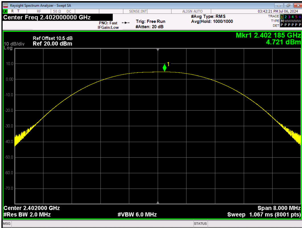
BLE_1M-Ant1-2402-PASS
