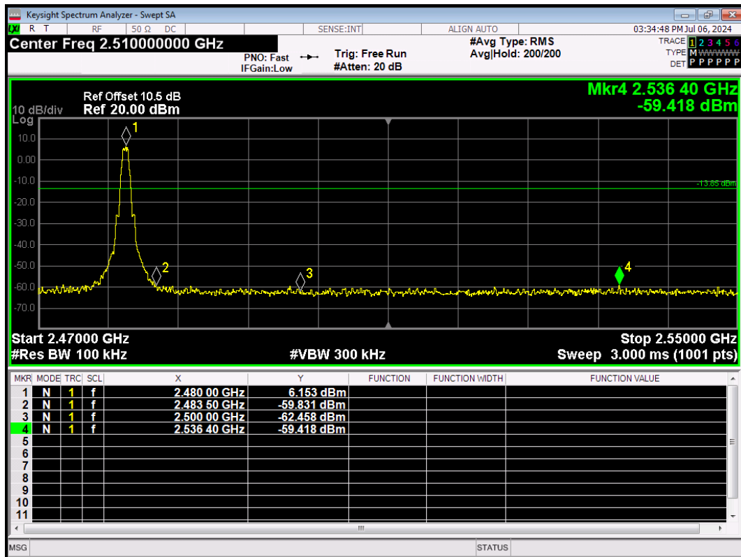
BLE_1M-Ant1-2480-PASS
