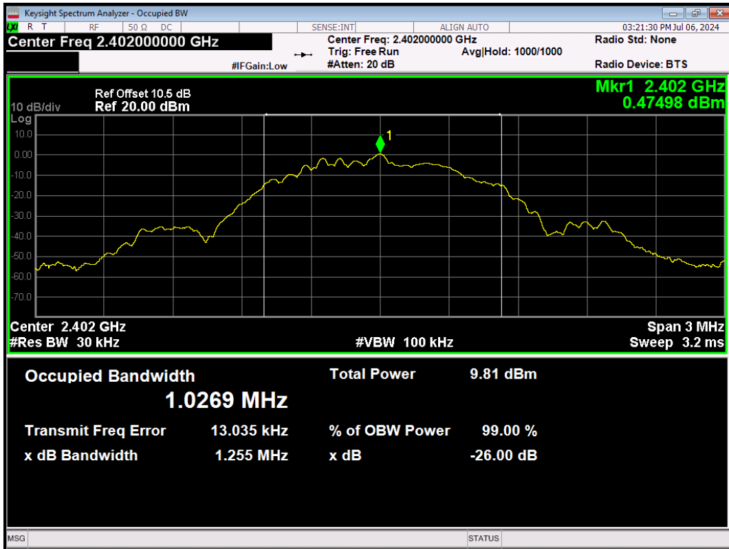
BLE_1M-Ant1-2402
