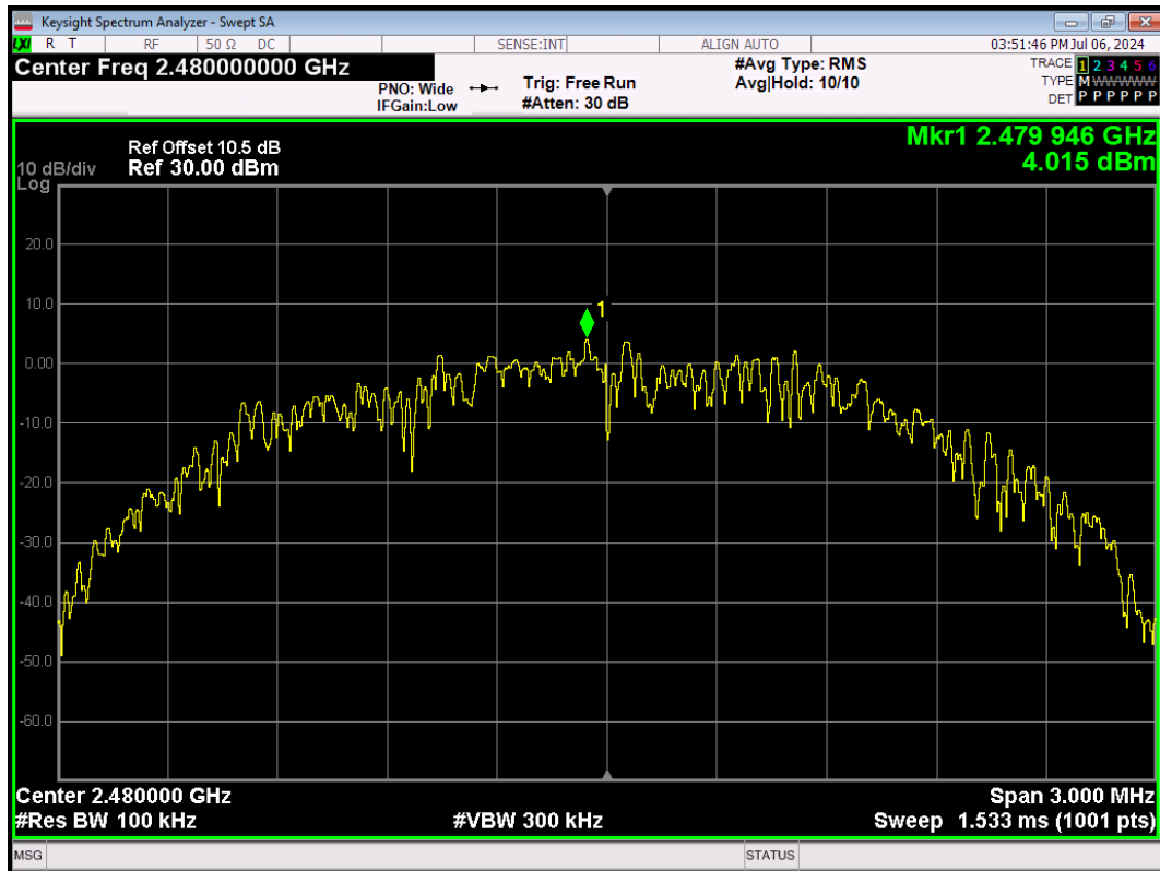
BLE_2M-Ant1-2480-0~Reference-PASS
