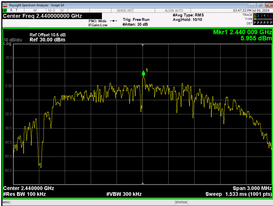
BLE_2M-Ant1-2440-0~Reference-PASS
