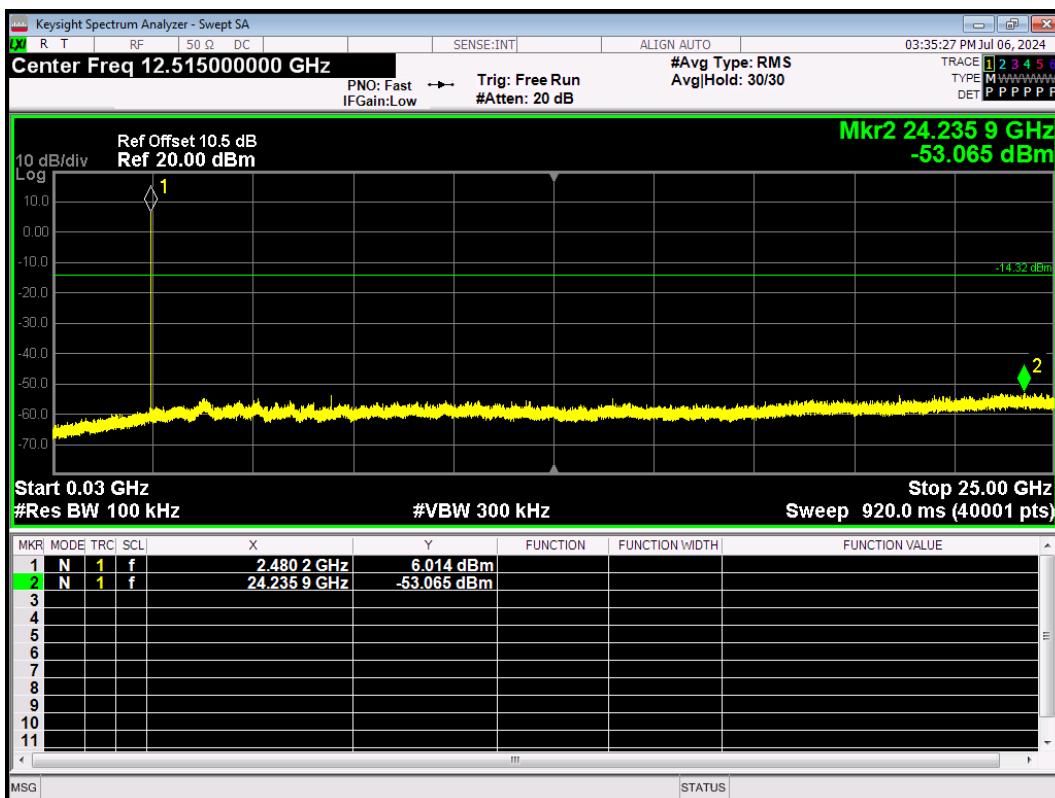
BLE_1M-Ant1-2480-30~25000-PASS
