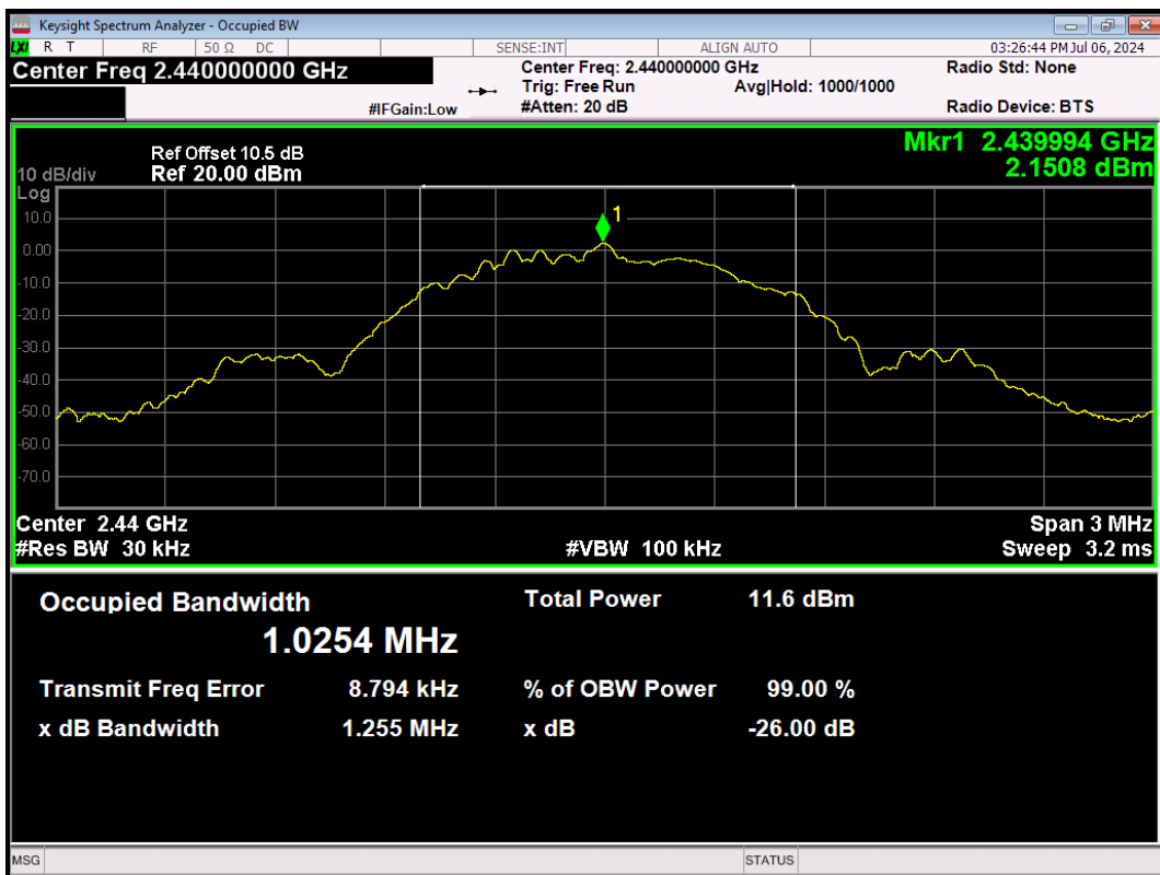
BLE_1M-Ant1-2440
