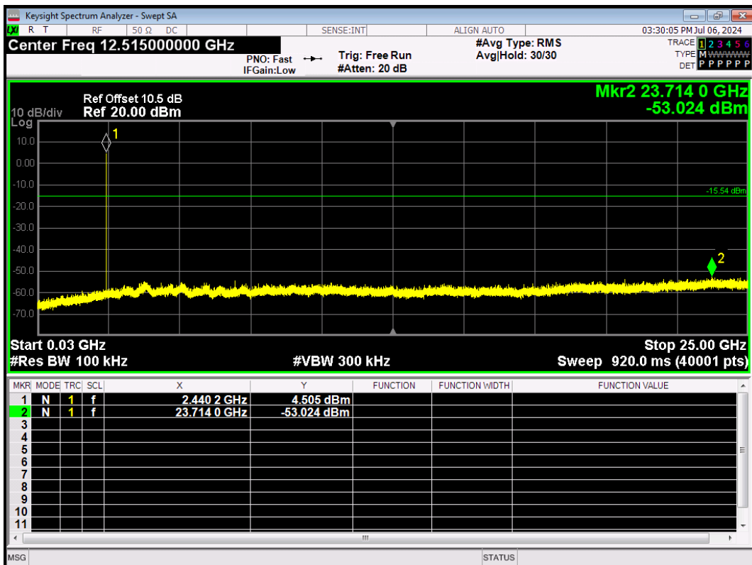
BLE_1M-Ant1-2440-30~25000-PASS
