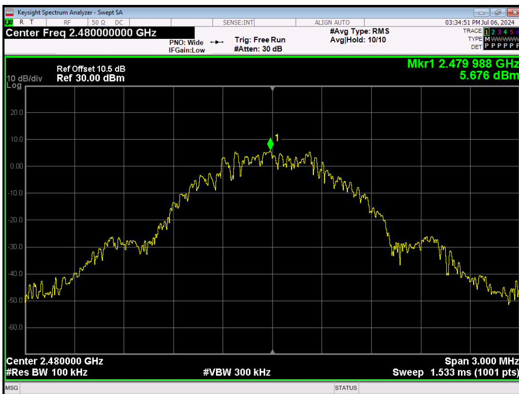
BLE_1M-Ant1-2480-0~Reference-PASS
