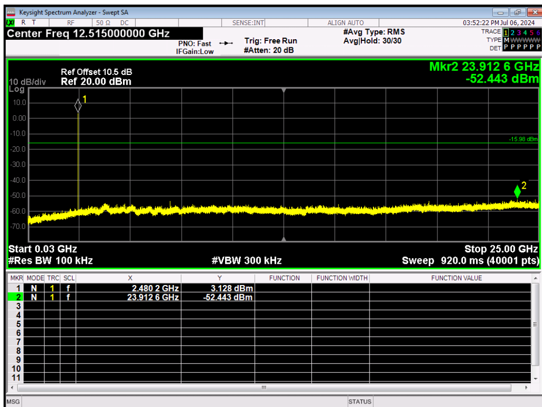
BLE_2M-Ant1-2480-30~25000-PASS
