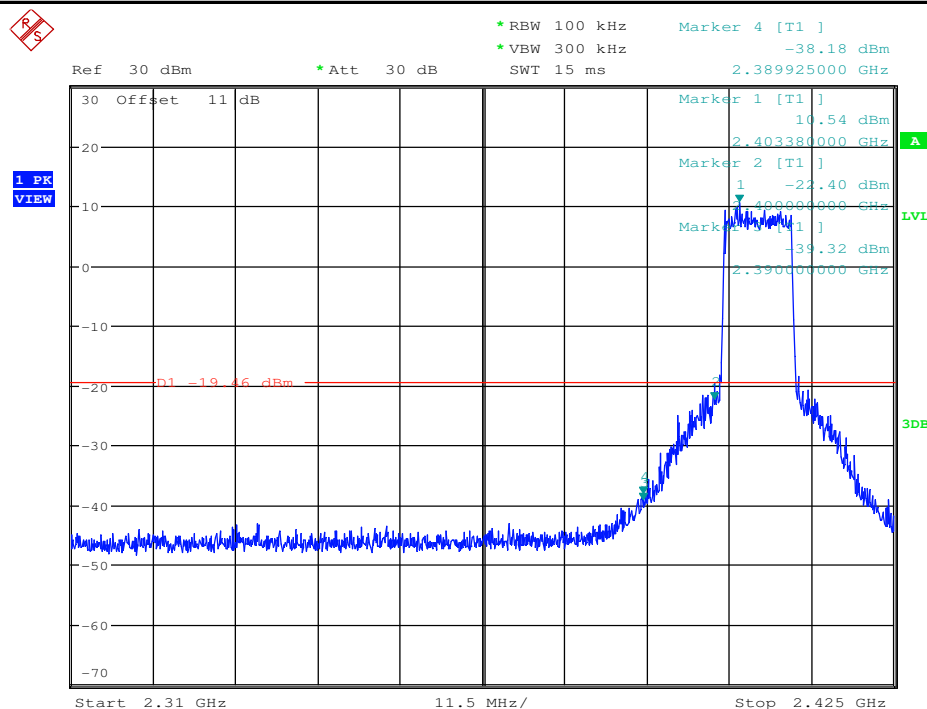
Band-edge for RF Conducted Emissions 10MHz 2406 Ant2
