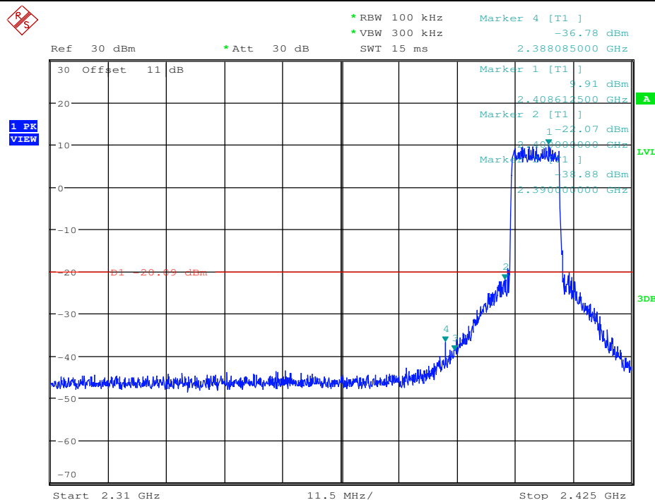
Band-edge for RF Conducted Emissions_10MHz_2406_Ant1
