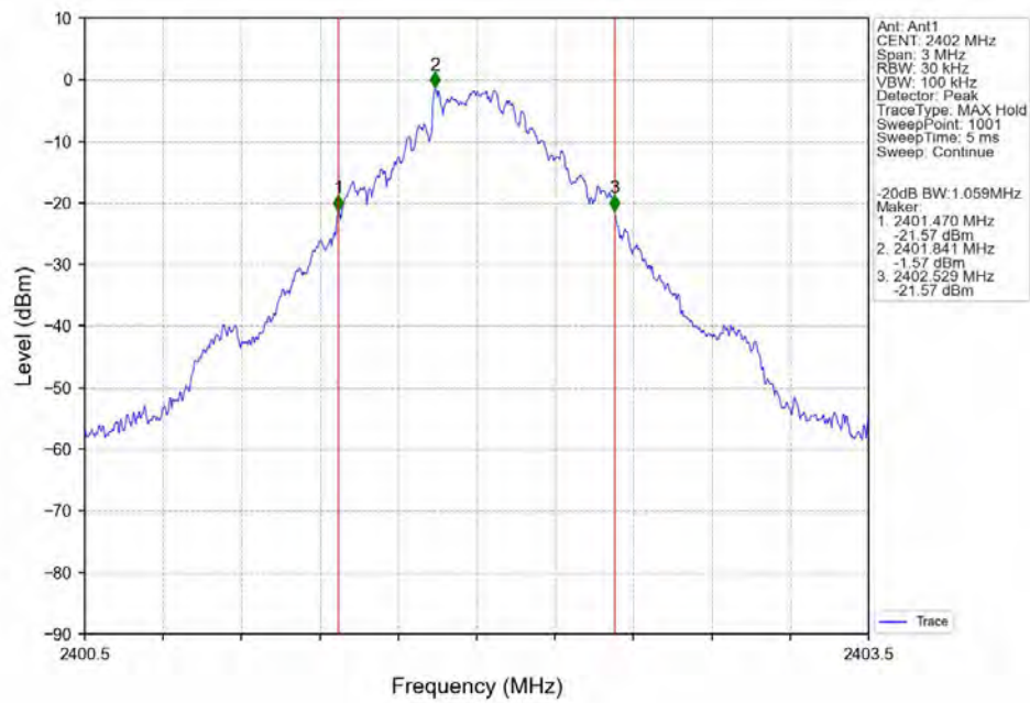
-20dB_Bandwidth_NVNT_ANT1_DH5_2402
