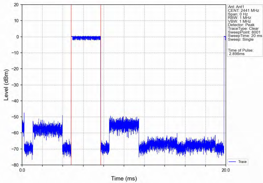
Dwell_Time_(Hopping)_NVNT_ANT1_2-DH5_2441_Accumulated
