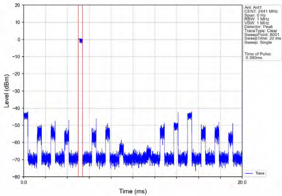
Dwell_Time_(Hopping)_NVNT_ANT1_2-DH1_2441_Accumulated
