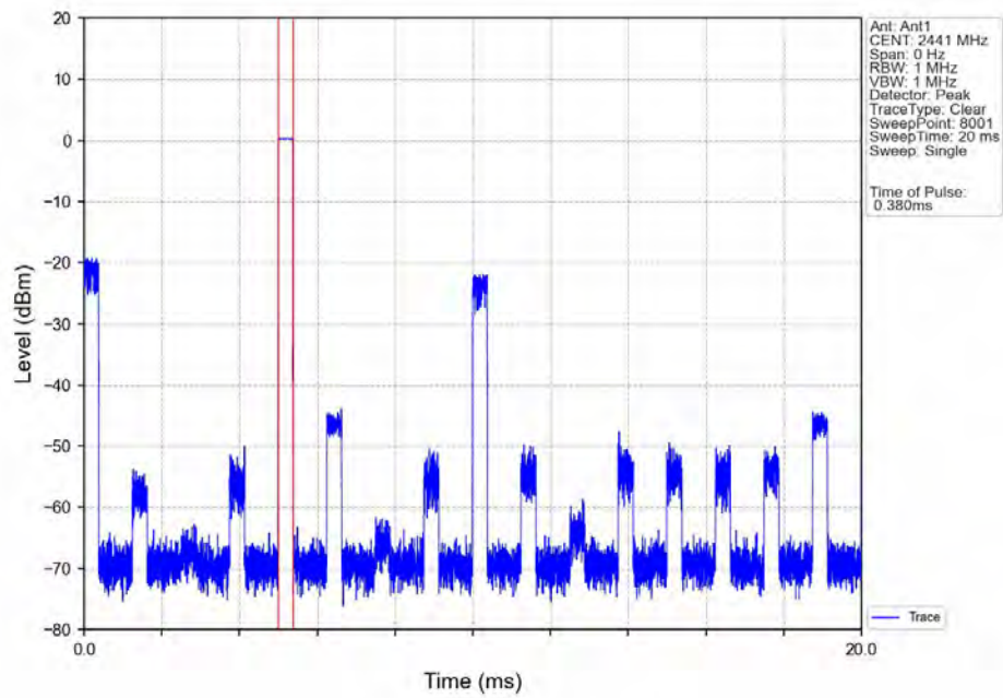
Dwell_Time_(Hopping)_NVNT_ANT1_1-DH1_2441_Accumulated
