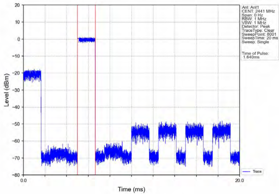
Dwell_Time_(Hopping)_NVNT_ANT1_3-DH3_2441_Accumulated
