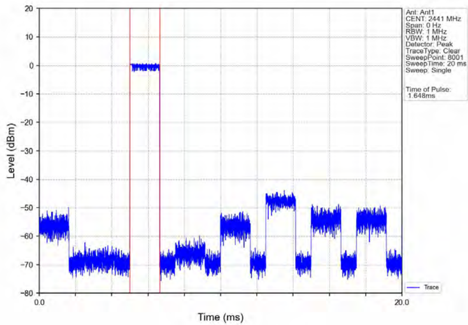
Dwell_Time_(Hopping)_NVNT_ANT1_2-DH3_2441_Accumulated
