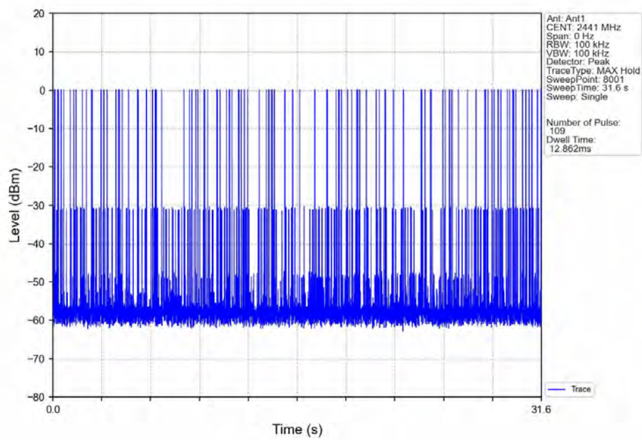
Dwell_Time_(Hopping)_NVNT_ANT1_3-DH5_2441_Accumulated
