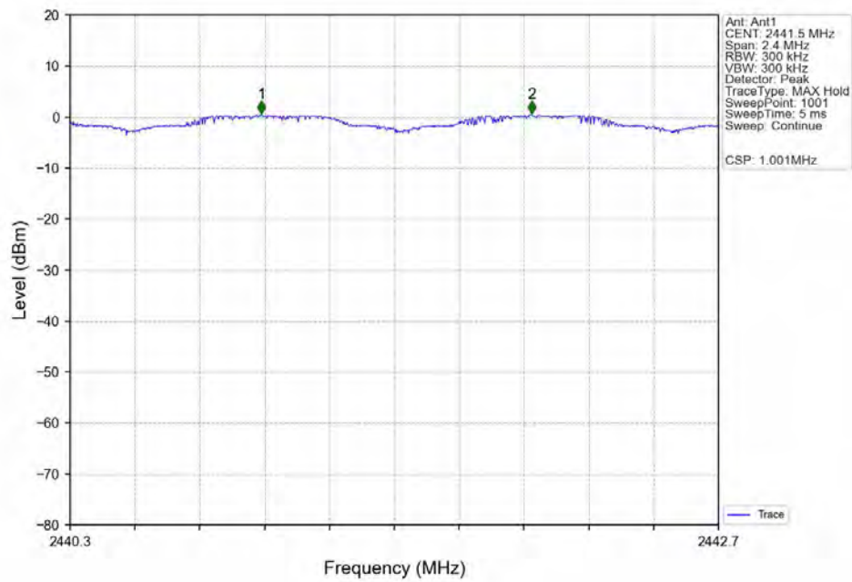
Carrier_Frequencies_Separation_(Hopping)_NVNT_ANT1_2DH5_Hopping
