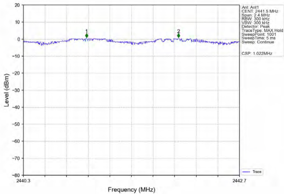
Carrier_Frequencies_Separation_(Hopping)_NVNT_ANT1_3DH5_Hopping
