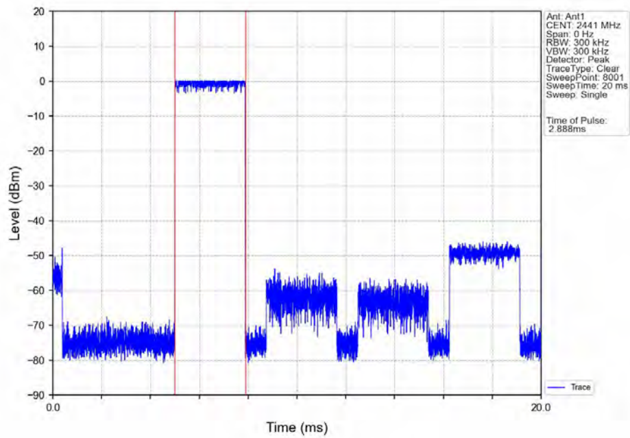
Dwell_Time_(Hopping)_NVNT_ANT1_DH5_2441_Accumulated
