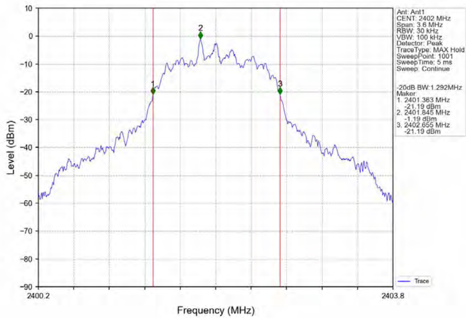
-20dB_Bandwidth_NVNT_ANT1_3-DH5_2402
