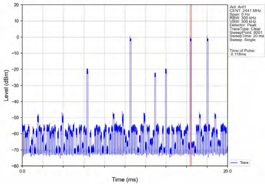
Dwell_Time_(Hopping)_NVNT_ANT1_3-DH5_2441_Accumulated
