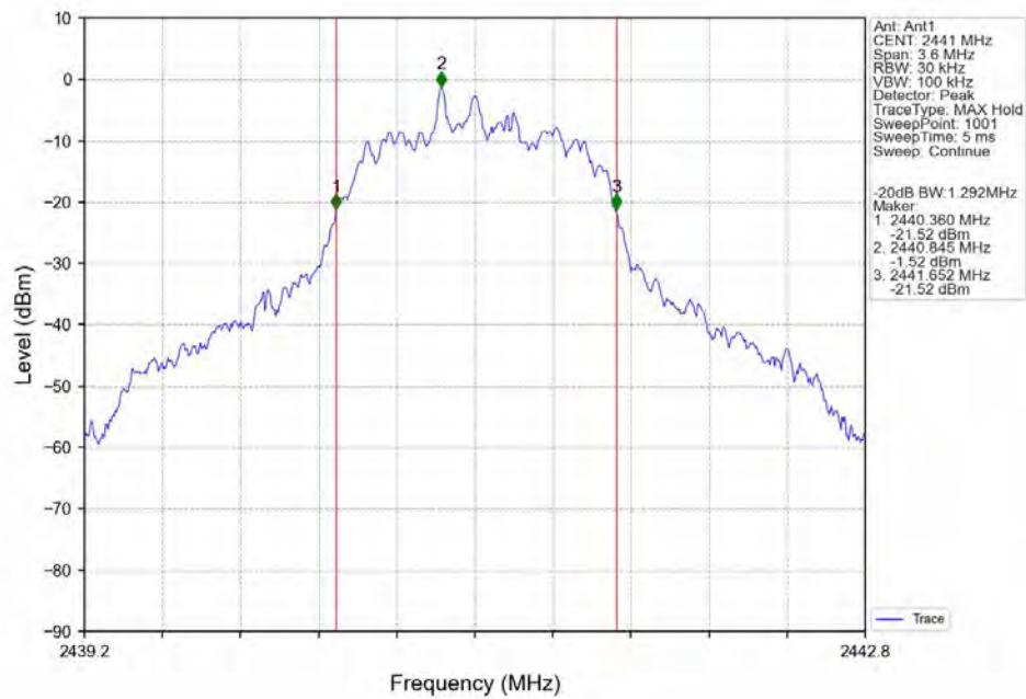
-20dB_Bandwidth_NVNT_ANT1_3-DH5_2441
