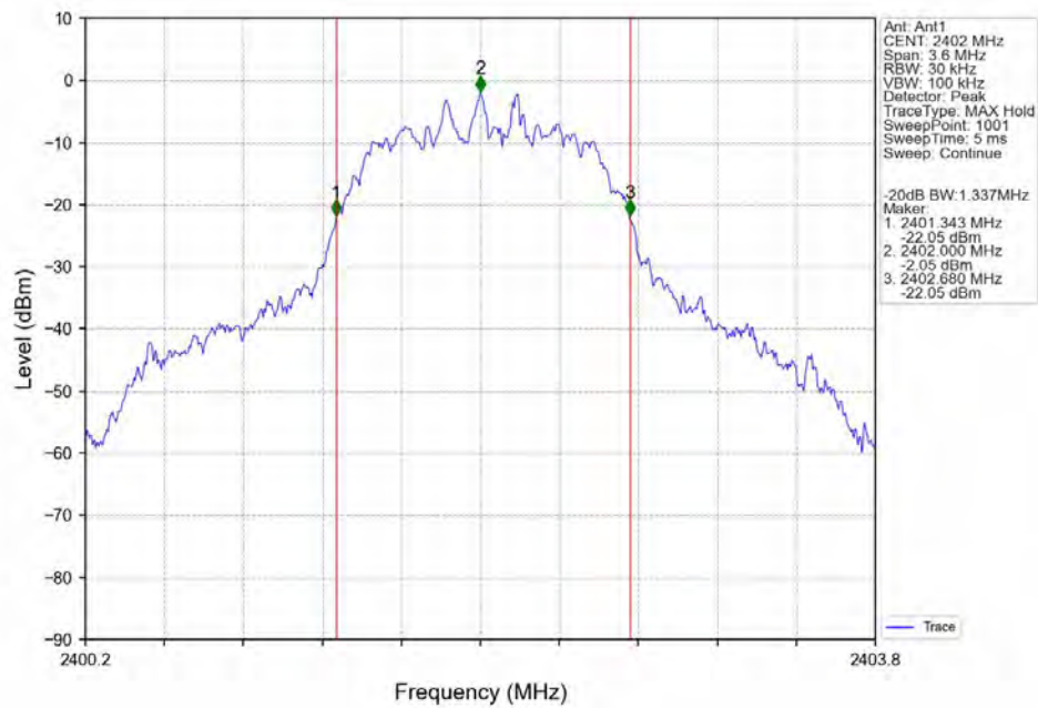
-20dB_Bandwidth_NVNT_ANT1_2-DH5_2402
