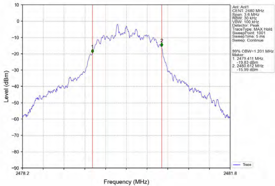
99%_Occupied_Bandwidth_NVNT_ANT1_3-DH5_2480
