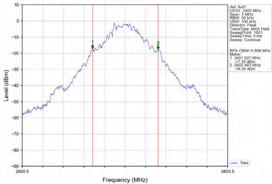
99%_Occupied_Bandwidth_NVNT_ANT1_DH5_2402
