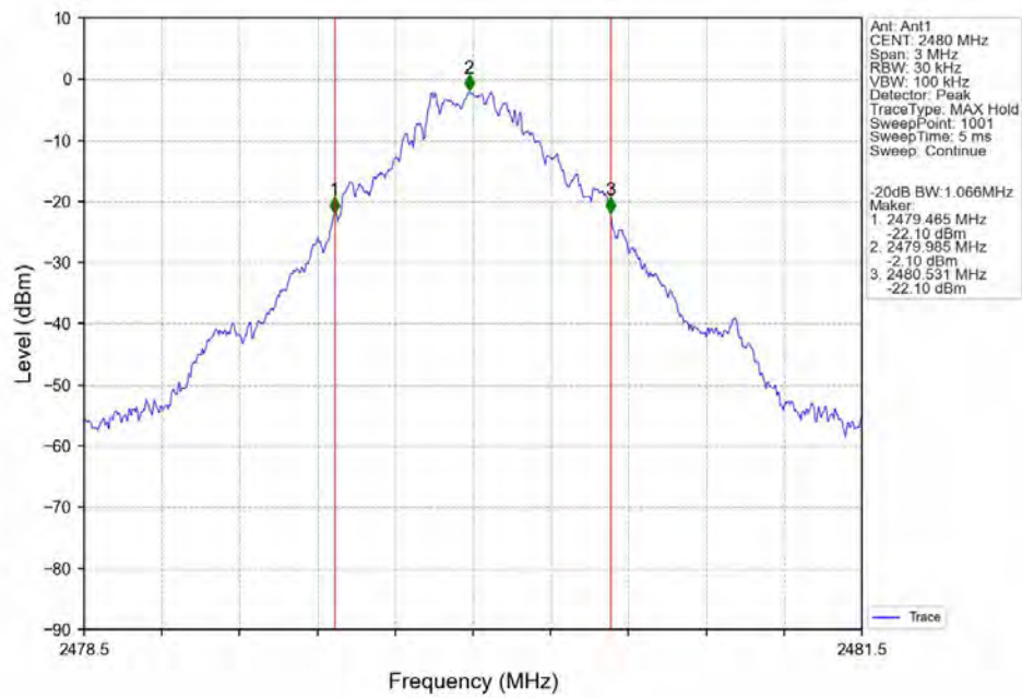
-20dB_Bandwidth_NVNT_ANT1_DH5_2480
