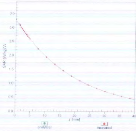
f = 850 MHz, WGLS R9 (H_convF)
