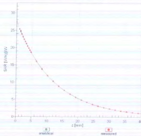
f = 1900 MHz, WGLS R22 (H_convF)
