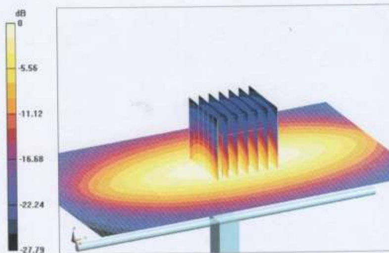
0 dB = 3.31 W/kg = 5.19 dBW/kg
