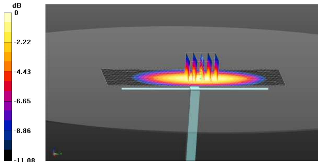
0 dB = 1.01 W/kg = 0.043 dBW/kg
