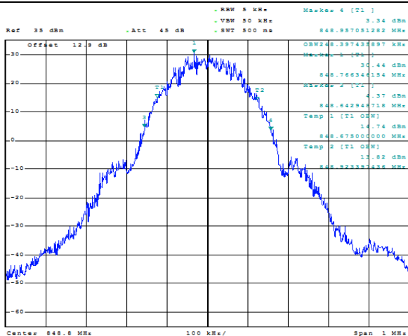
Channel 190
