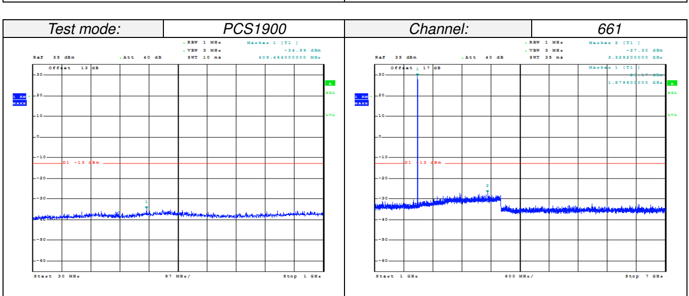
30MHz~1GHz
