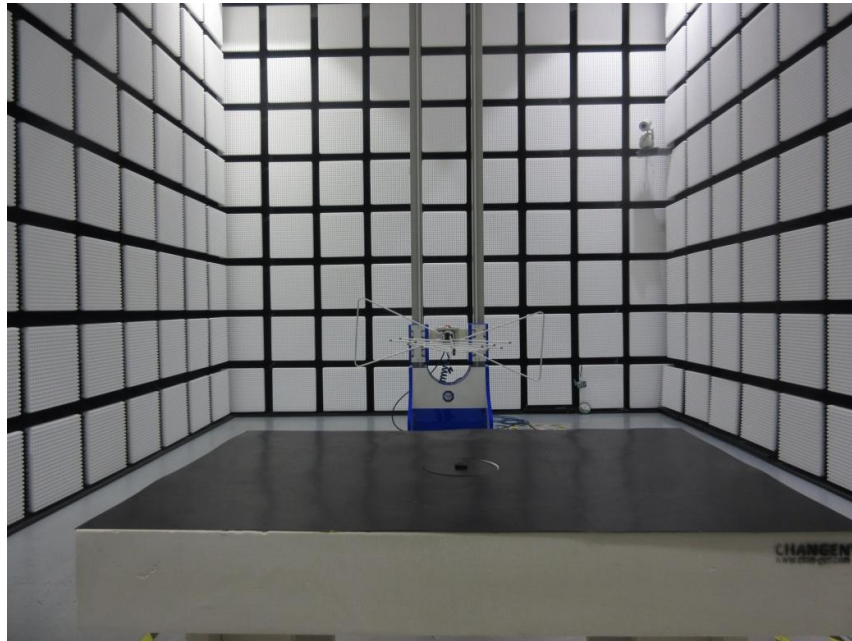
Radiated Spurious emission test below 1GHz
