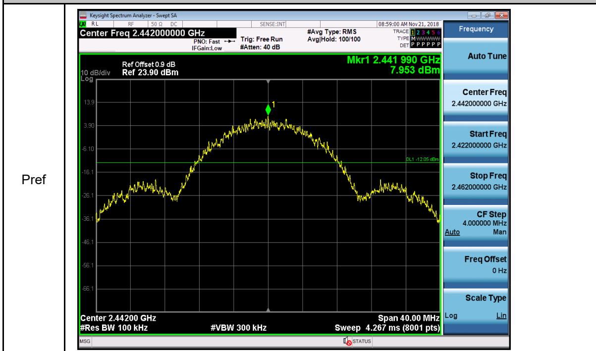
RF Conducted Spurious Emissions_11B_2442_Ant1
