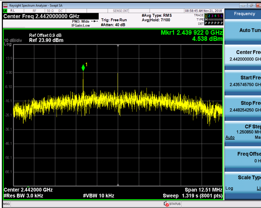
Maximum Peak power spectral density_11B_2442_Ant1
