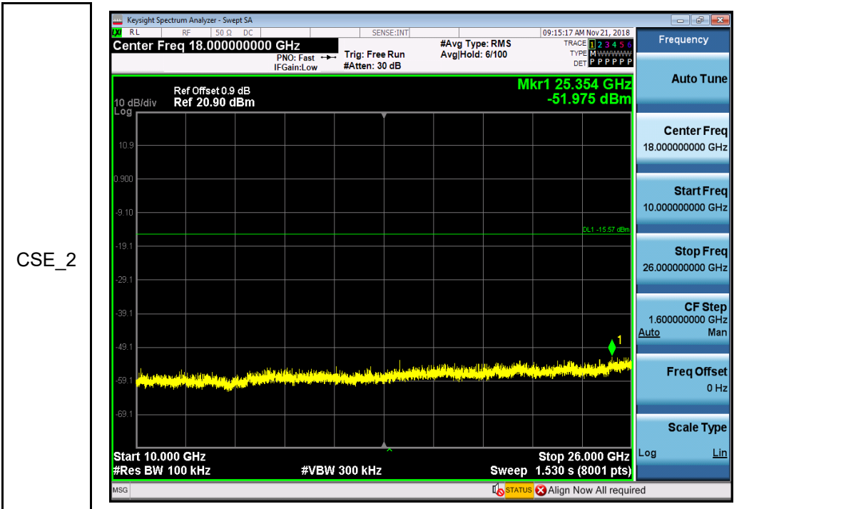
RF Conducted Spurious Emissions_11N20SISO_2442_Ant1
