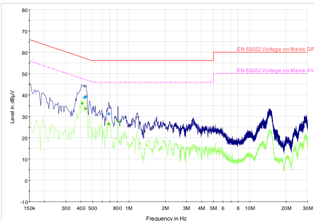
— EN 55022 Voltage on Mains QP - - - EN 55022 Voltage on Mains AV — Preview Result 1-PK+ — Preview Result 2-AVG ◆ Final Result 1-QPK ◆ Final Result 2-AVG
