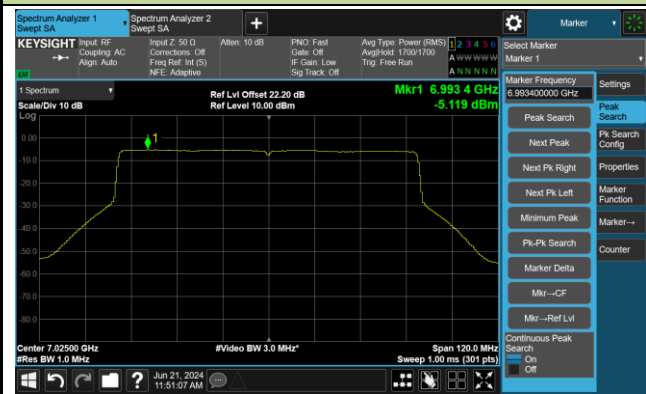
Channel 215 (7025MHz)
