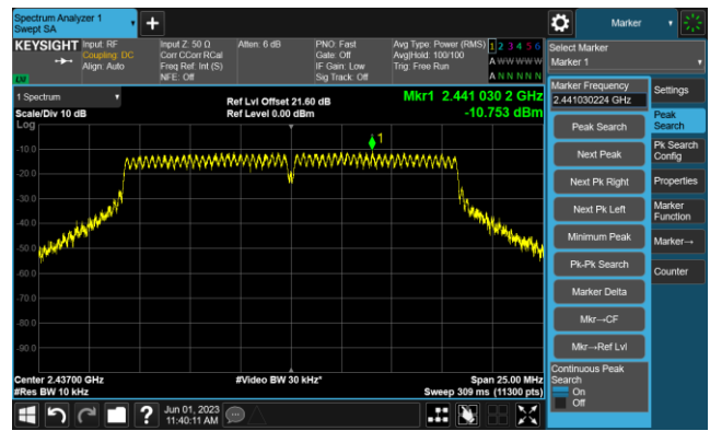
Channel 06 (2437MHz)
