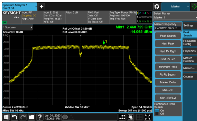
Channel 09 (2452MHz)
