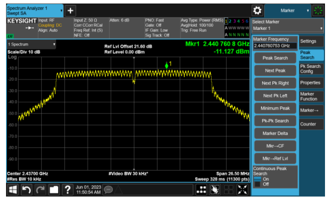
Channel 06 (2437MHz)
