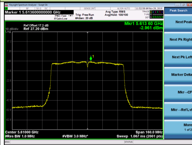
Channel 122 (5610MHz)
