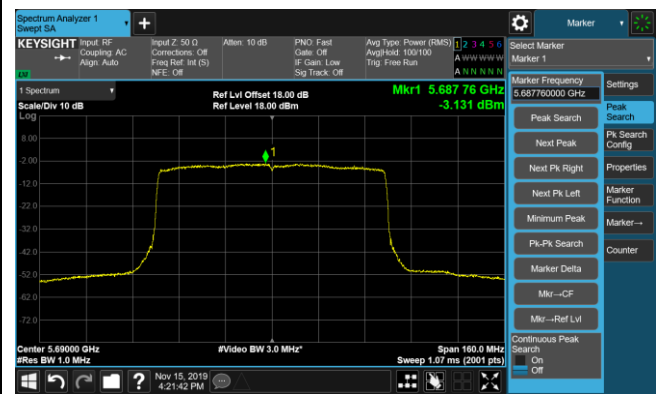
Channel 138 (5690MHz)
