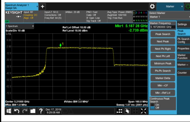
Channel 42 (5210MHz)
