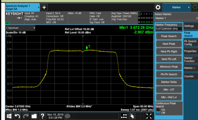
Channel 134 (5670MHz)
