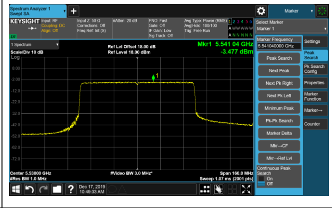
Channel 106 (5530MHz)
