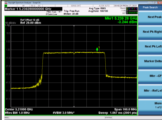
Channel 42 (5210MHz)
