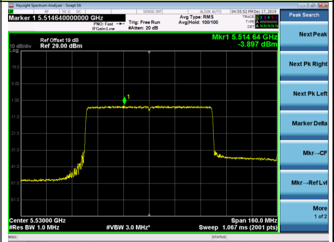
Channel 106 (5530MHz)
