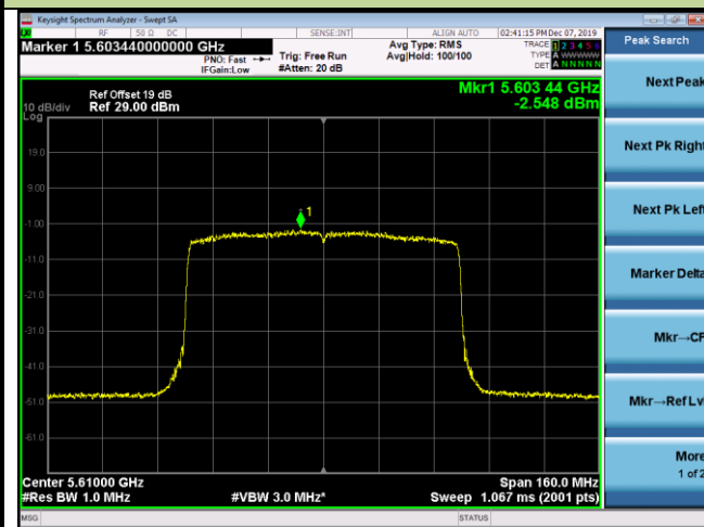
Channel 122 (5610MHz)
