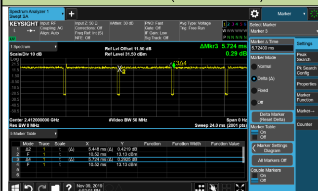
802.11ax-HE20 (T = 5.448 ms)
