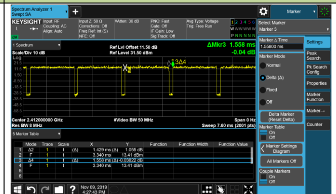
802.11n-HT40 (T = 5.412 ms)
