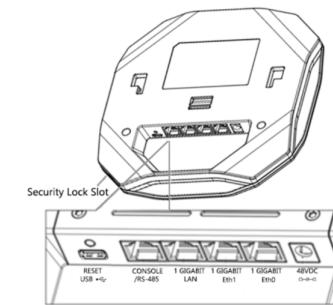
Figure 3: OAW-AP1331 Back View
