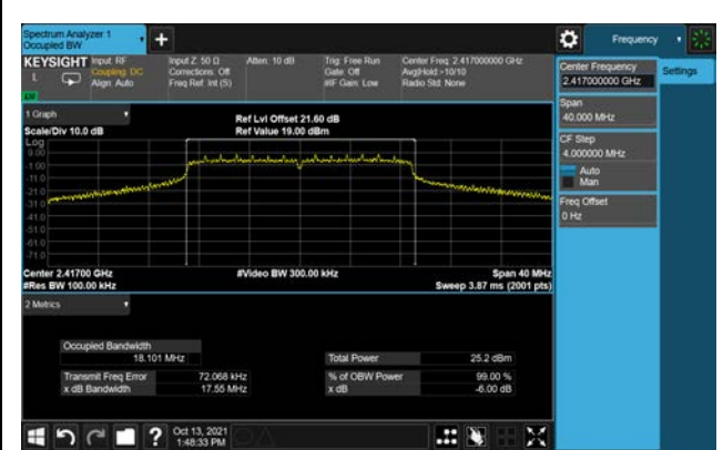
Channel 02 (2417MHz)
