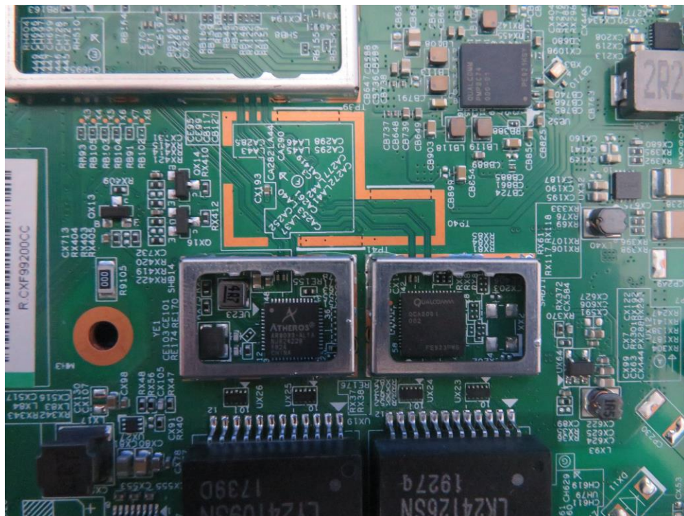
(14) EUT Photo_OAW-AP1322
