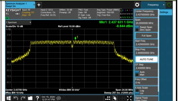
Channel 06 (2437MHz)
