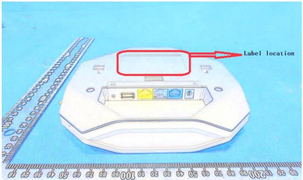
Label location
