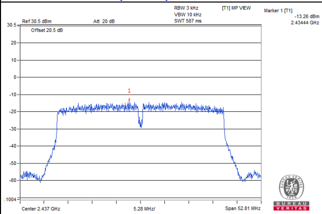
802.11n (40MHz) / Chain 2: CH6
