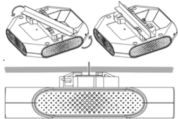
Figure 5: Mounting AP
