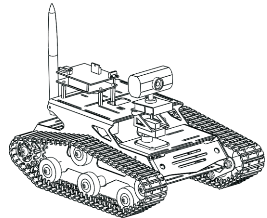
Arduino version TH Robot finished photograph
