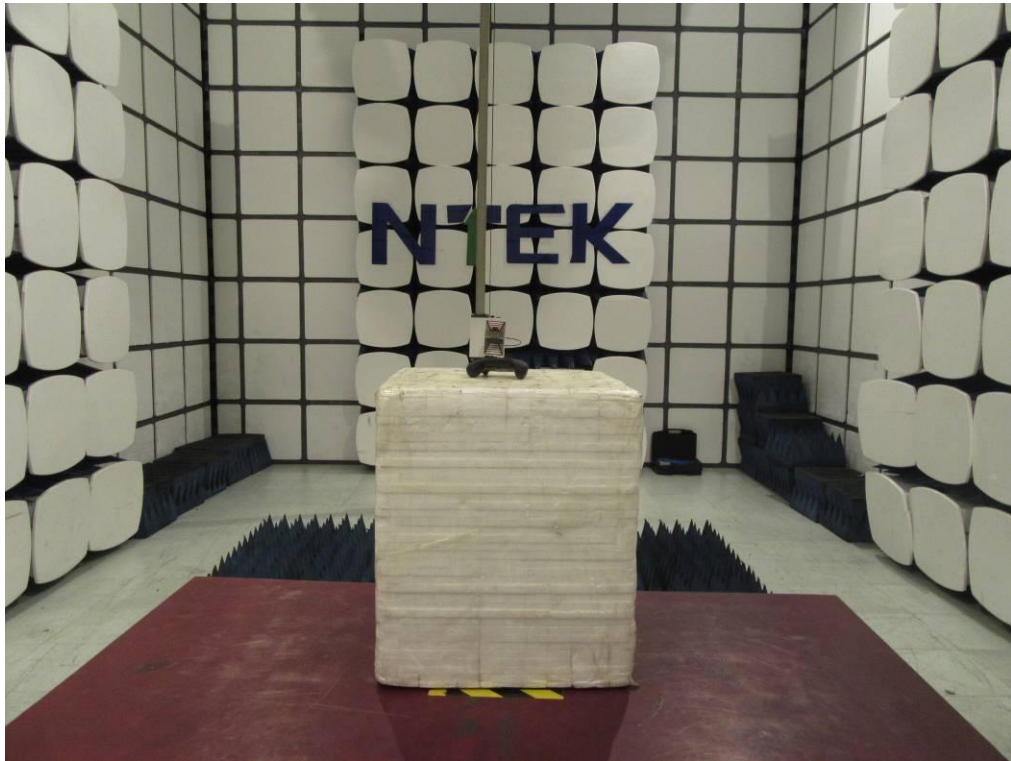
Photo 3 Radiated Measurement(Above 1GHz)
