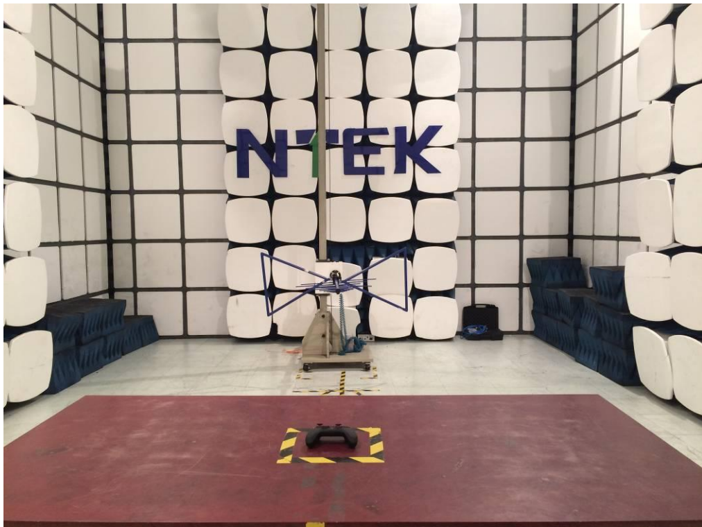
Photo 2 Radiated Measurement(30MHz~1GHz)
