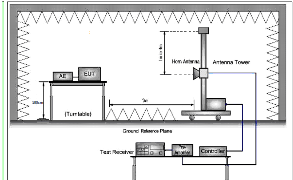
Above 1 GHz
