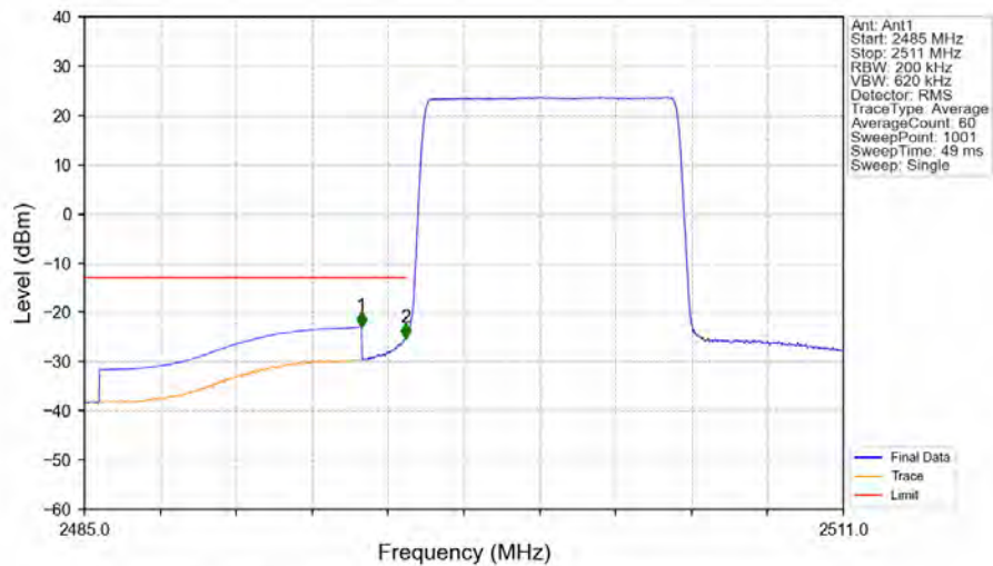
41_Single_NTNV_CC1:10MHz_QPSK_CC1:2501MHz_Ant1
