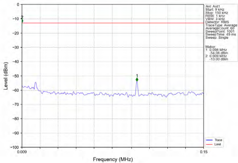
41_Single_NTNV_CC1:5MHz_QPSK_CC1:2687.5MHz_Ant1
