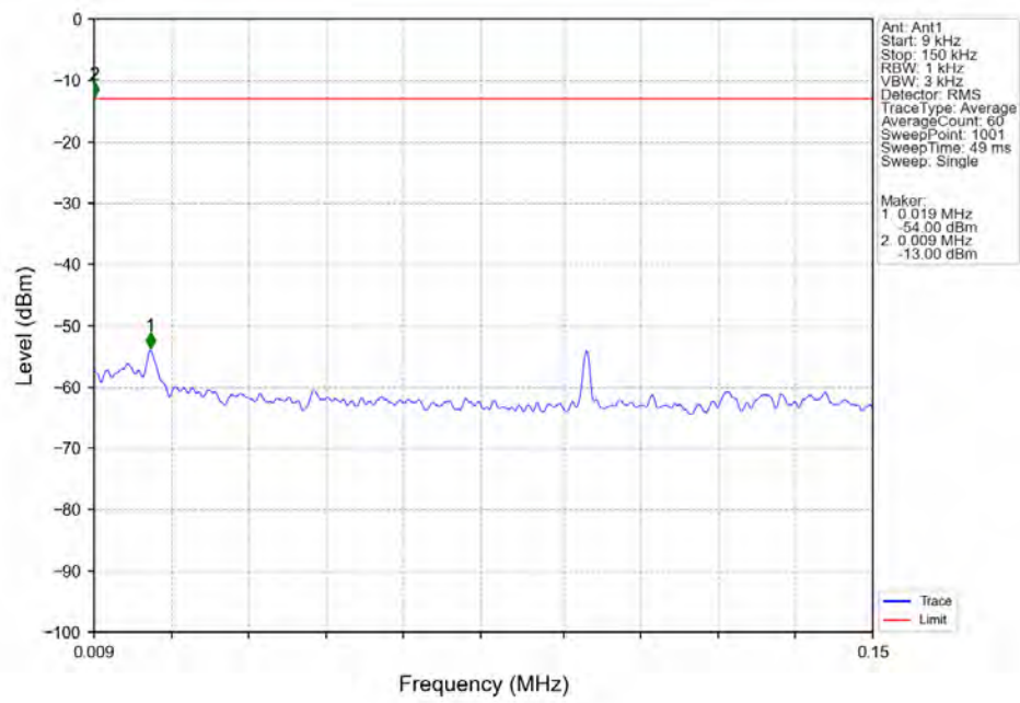
41_Single_NTNV_CC1:5MHz_64QAM_CC1:2593MHz_Ant1
