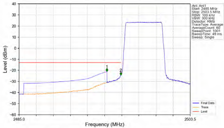
41_Single_NTNV_CC1:5MHz_64QAM_CC1:2498.5MHz_Ant1
