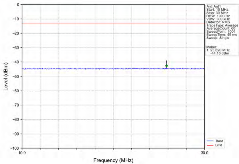
41_Single_NTNV_CC1:5MHz_256QAM_CC1:2498.5MHz_Ant1
