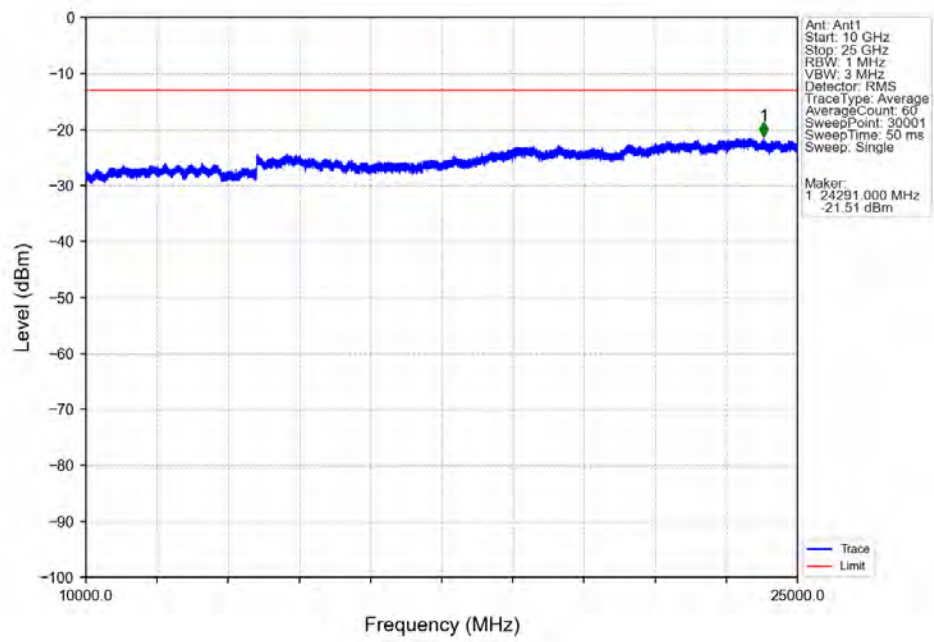
41_Single_NTNV_CC1:5MHz_QPSK_CC1:2498.5MHz_Ant1
