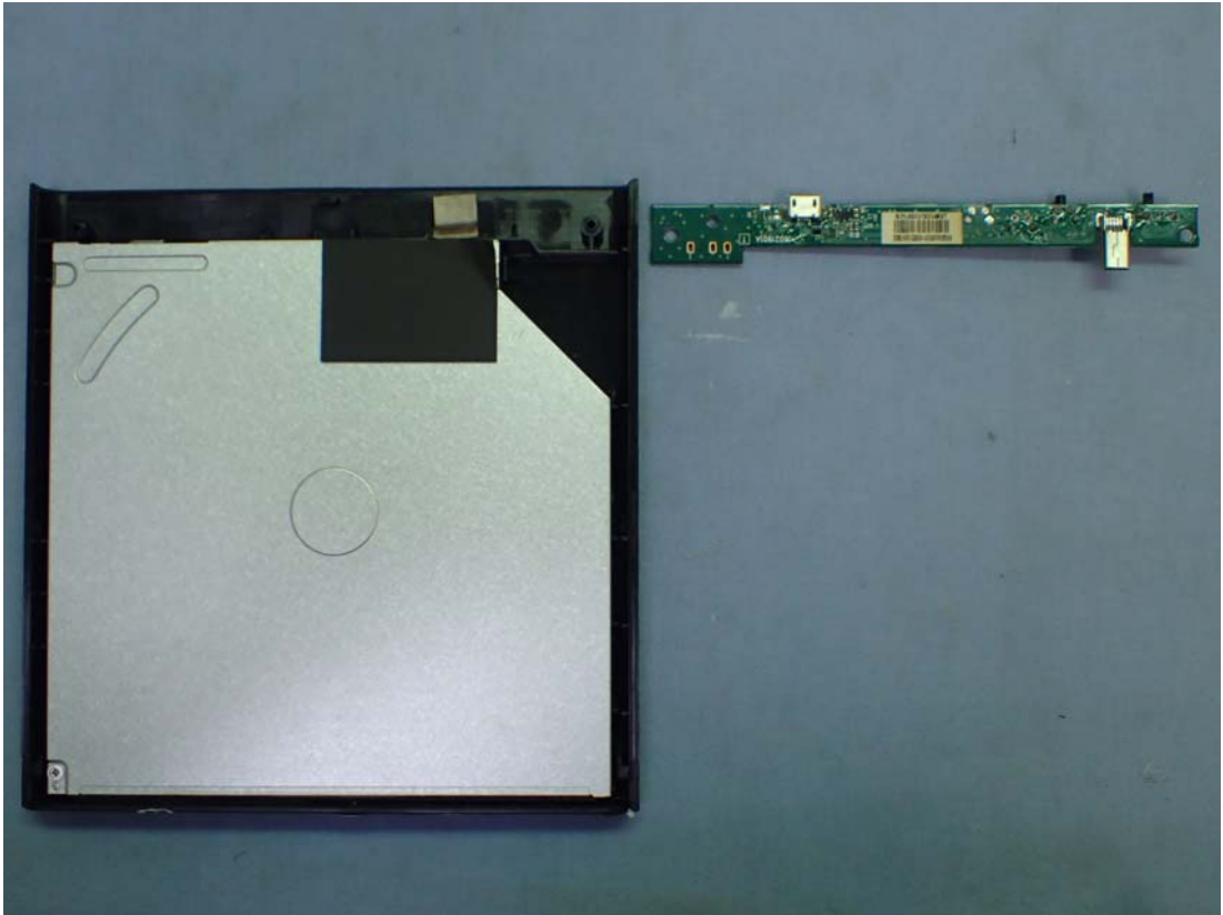
Figure 8 Internal View (Remove DVD/CD Drive)
