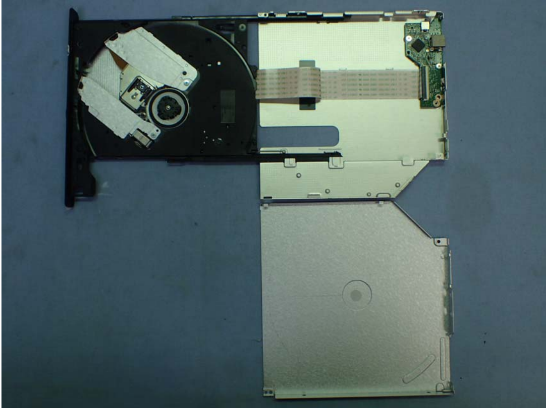
Figure 14 Internal View
