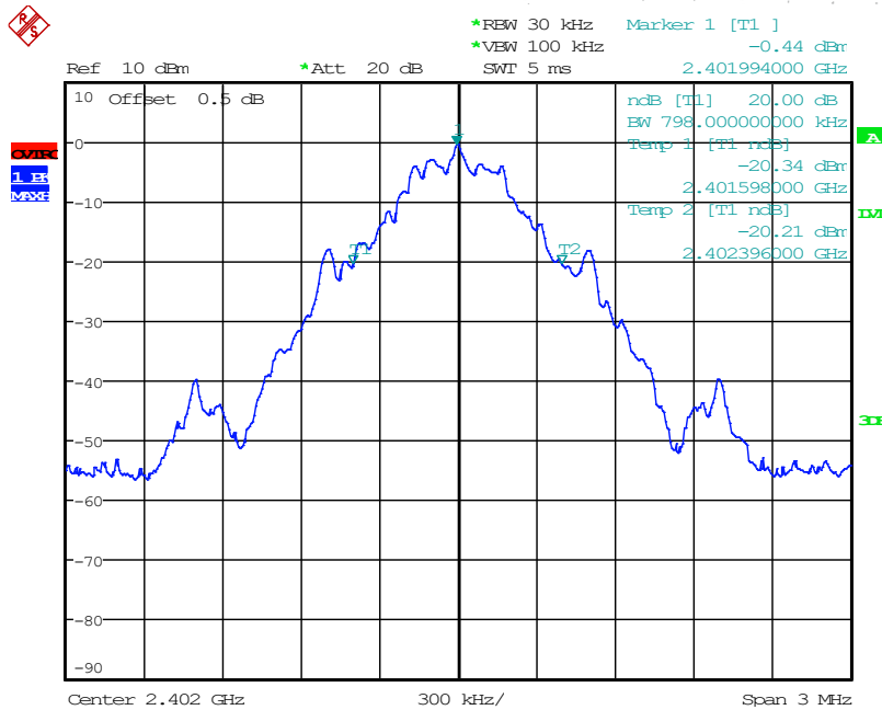
Test plots GFSK Low Channel
