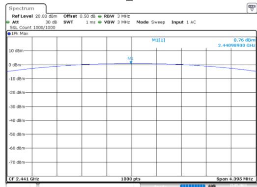
GFSK_Middle
