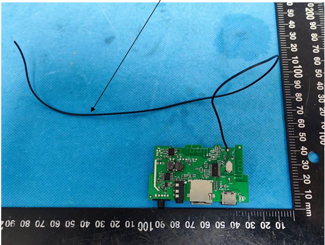
FM Antenna
