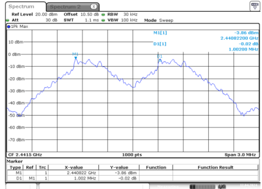
GFSK_Mid_DH1
