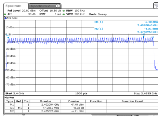
PI/4-DQPSK_Hopping_2DH1
