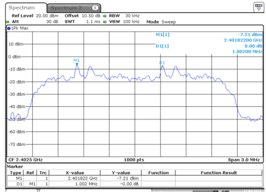
PI/4-DQPSK_Low_2DH1
