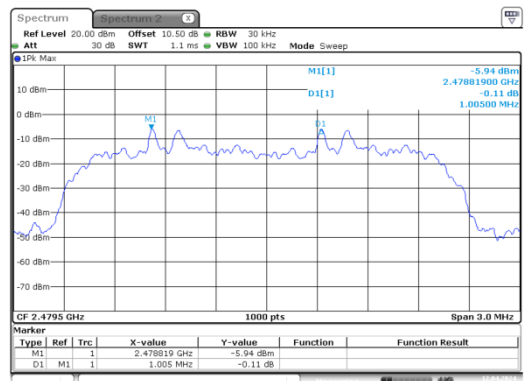
PI/4-DQPSK_High_2DH1
