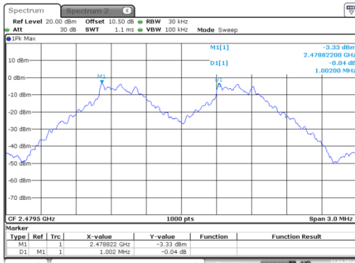
GFSK_High_DH1
