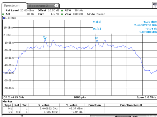
PI/4-DQPSK_Mid_2DH1
