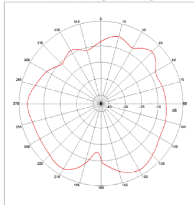
Far-field Power Distribution(H+V) on X-Z Plane Plot Peak Gain(H+V)= 1.9 dBi, Plot AvgGain(H+V)= -3.83dBi @2.4000 GHz
