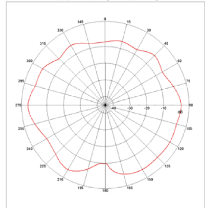
Far-field Power Distribution(H+V) on Y-Z Plane Plot Peak Gain(H+V)= 1.11 dBi, Plot AvgGain(H+V)= -2.95dBi @2.4000 GHz
