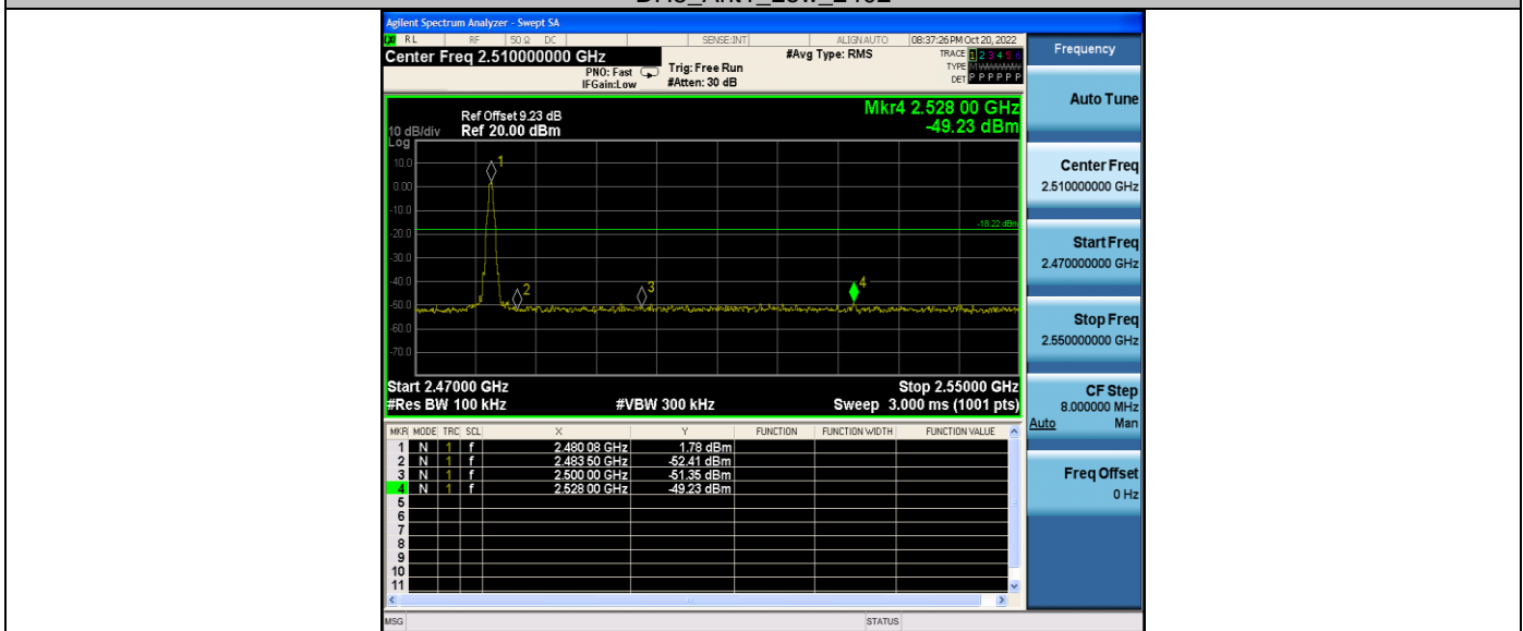
DH5_Ant1_High_2480
