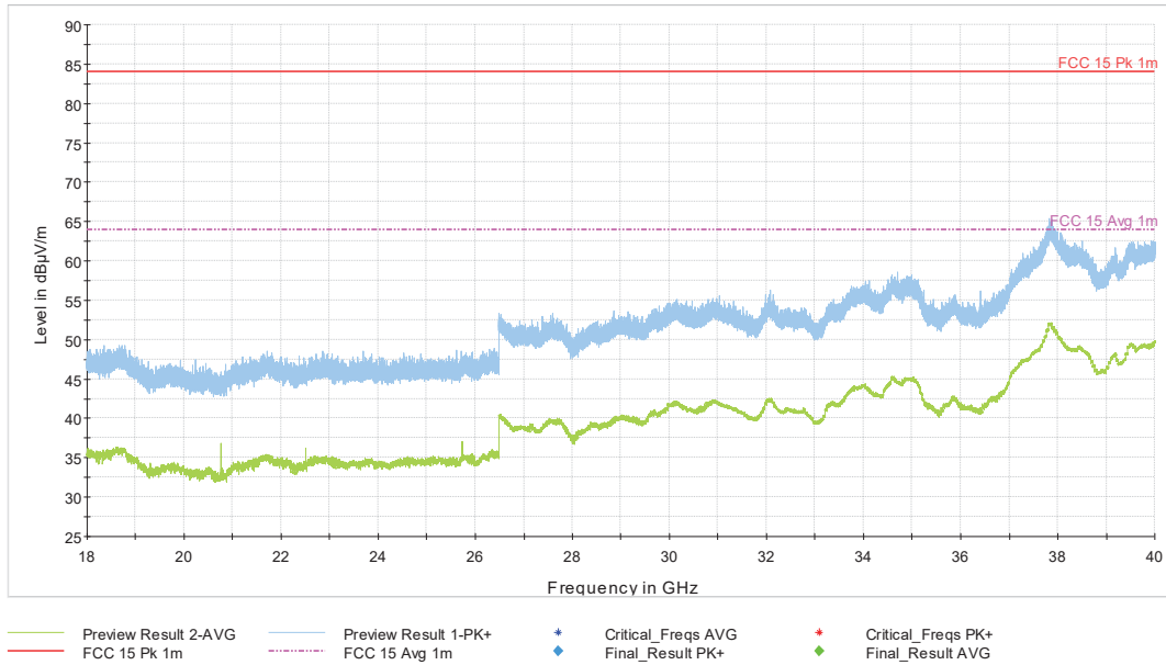
Figure 103: 18-40GHz 802.11n HT40 Mode Channel 38
