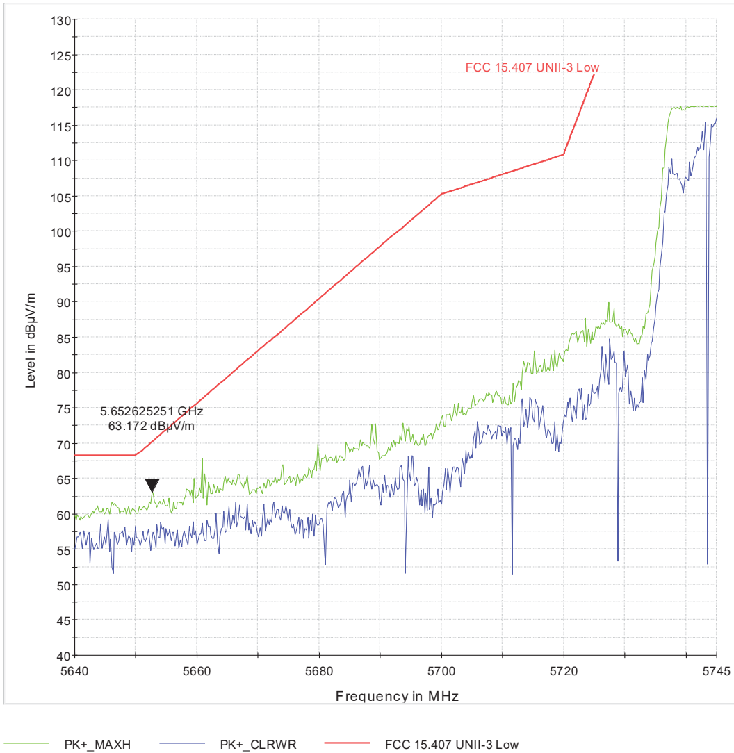
Figure 65: Low U-NII-3 band edge for 802.11n HT40+ MCS0 at Channel 151
