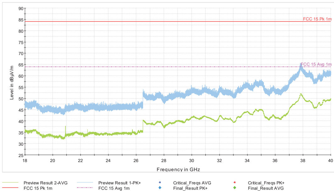
Figure 104: 18-40GHz 802.11n HT40 Mode Channel 46
