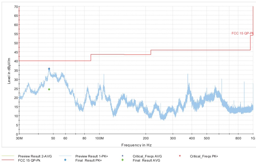
Figure 98: 30MHz-1GHz 802.11n HT40 Mode Channel 46
