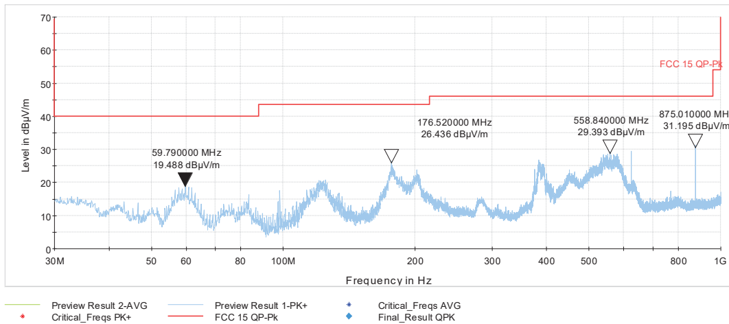
Figure 141: 30MHz-1GHz 802.11ac VHT80+80 Mode Channel 42 & 155
