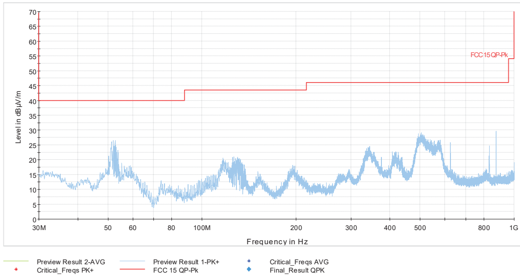
Figure 84: 30MHz-1GHz 802.11a Mode Channel 44
