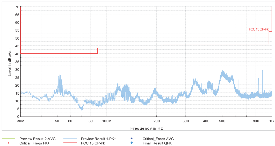
Figure 85: 30MHz-1GHz 802.11a Mode Channel 48
