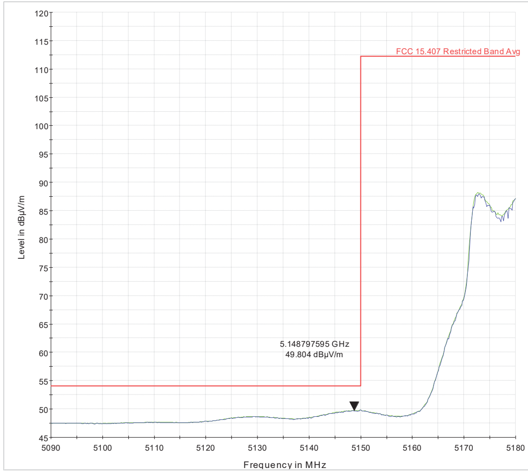
Figure 62: UNII-1 Low Band Edge for 802.11ac VHT80+80 MCS0 at 5210 & 5775 MHz-A verage
