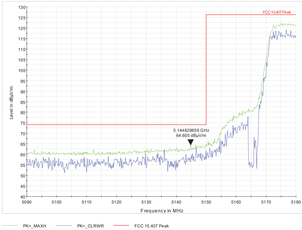
Figure 57: UNII-1 Low Band Edge for 802.11ac VHT20 MCS0 at 5180 MHz-Peak
