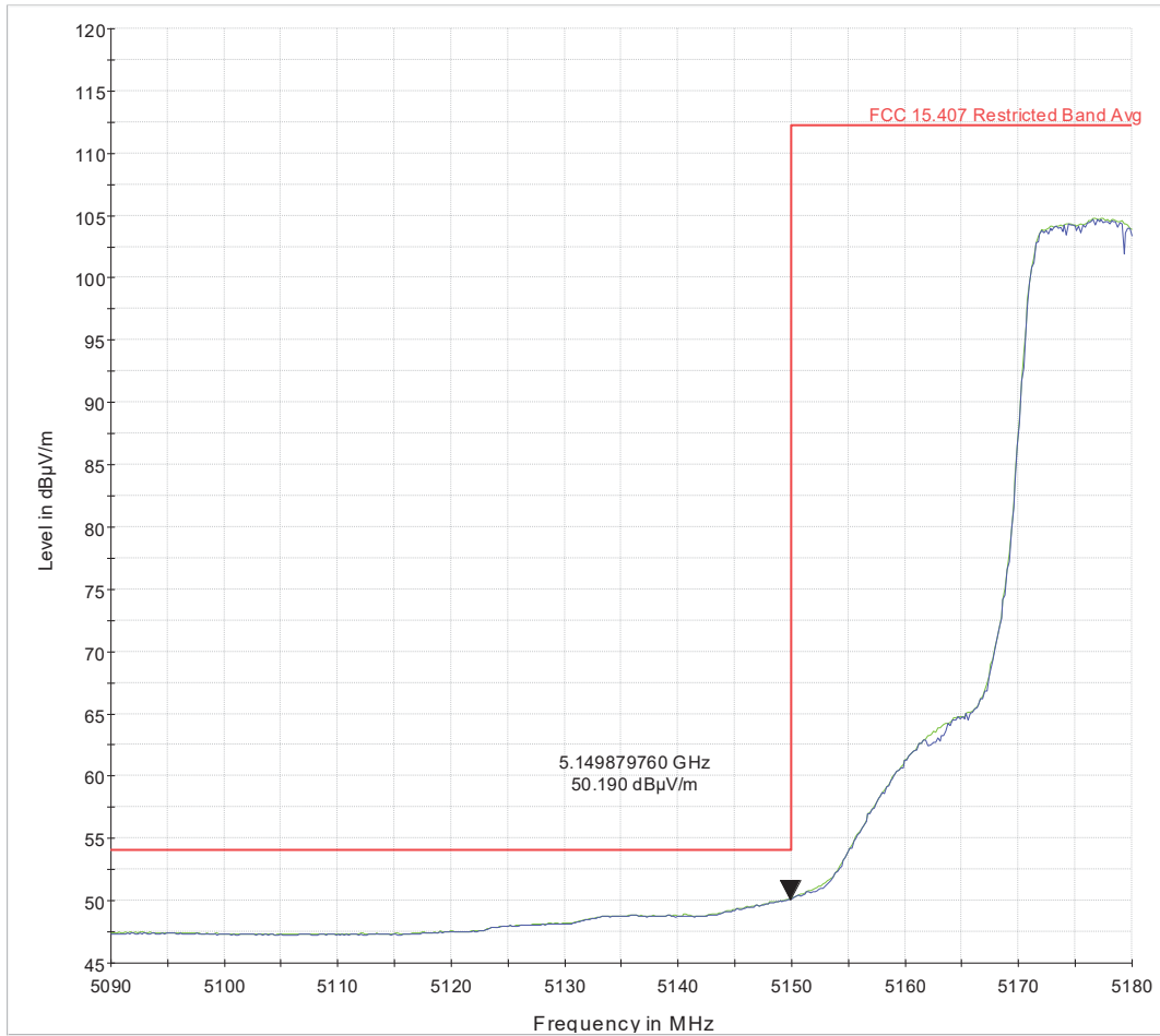
Figure 56: UNII-1 Low Band Edge for 802.11ac VHT20 MCS0 at 5180 MHz-Average
