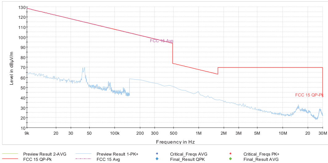
Figure 105: 9KHz-30MHz 802.11ac VHT80 Mode Channel 42
