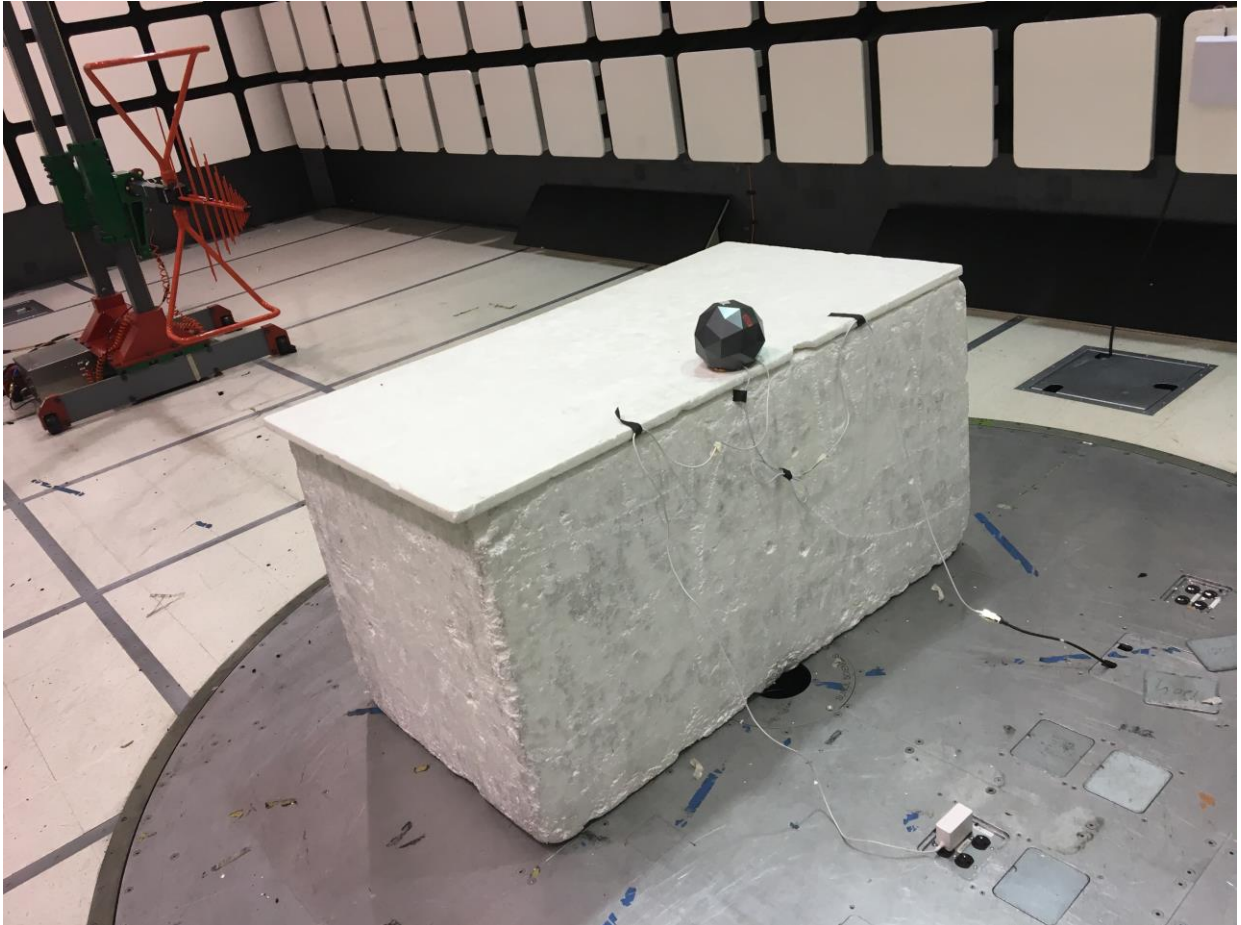
Figure 2: Test Setup for Radiated Emissions 30 MHz to 1000 MHz (CDD and BT LE Modes)
