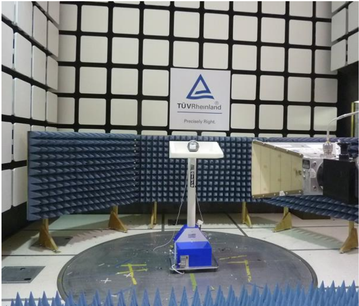
Figure 7: Test Setup for Radiated Band Edge (CDD & BT LE Modes)
