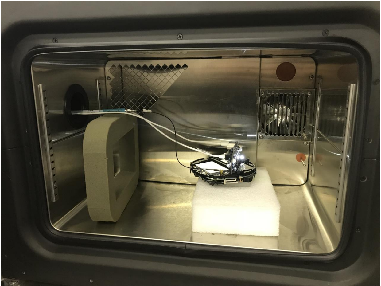
Figure 12: Test Setup for Conducted Emissions (Antenna Port- BT LE)
