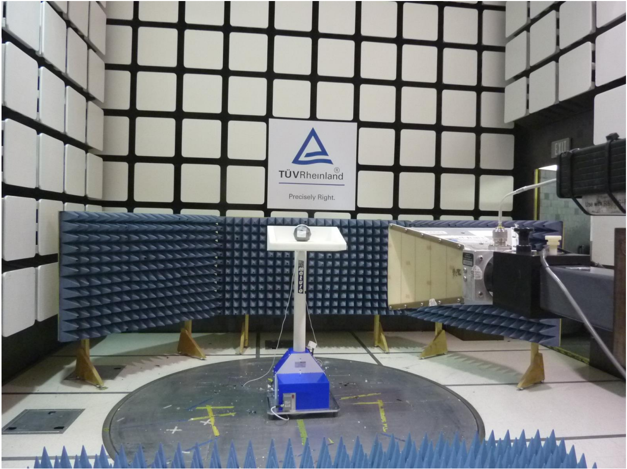
Figure 3: Test Setup for Radiated Emissions 1 GHz to 18 GHz – Front (CDD and BT LE Modes)
