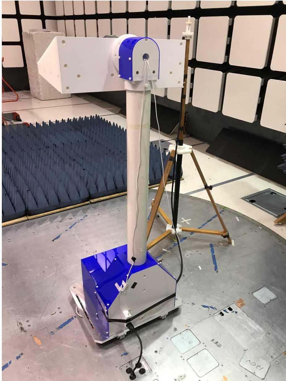
Figure 4: Test Setup for Radiated Emissions 1 GHz to 18 GHz – Rear (Beamforming Mode)
