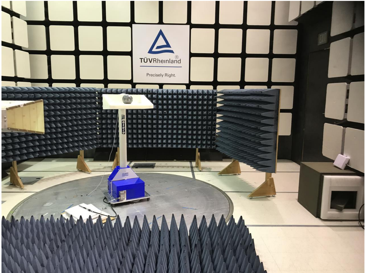
Figure 8: Test Setup for Radiated Band Edge (Beamforming Mode)
