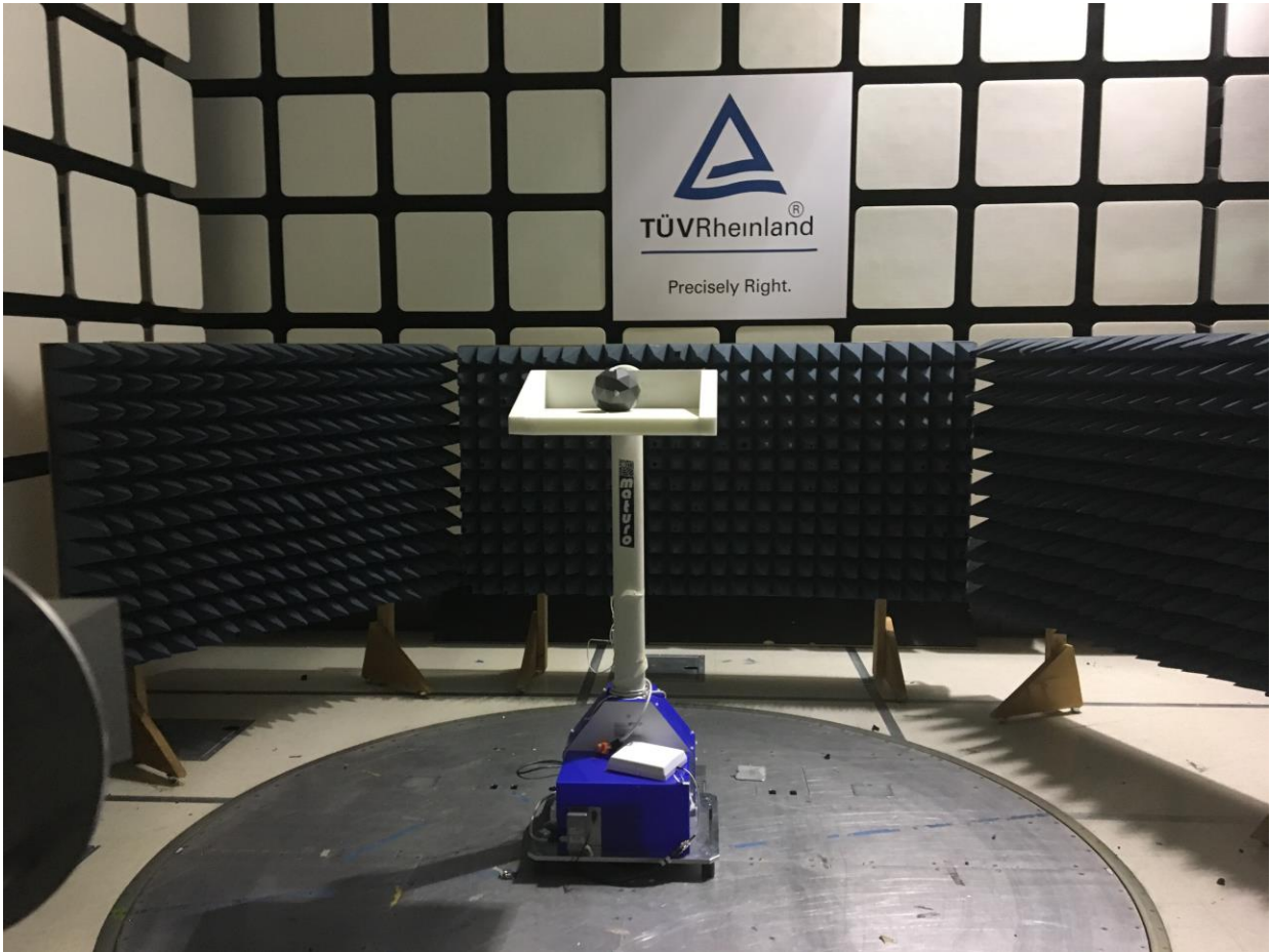
Figure 5: Test Setup for Radiated Emissions 18 GHz to 26.5 GHz (CDD and BT LE Modes)
