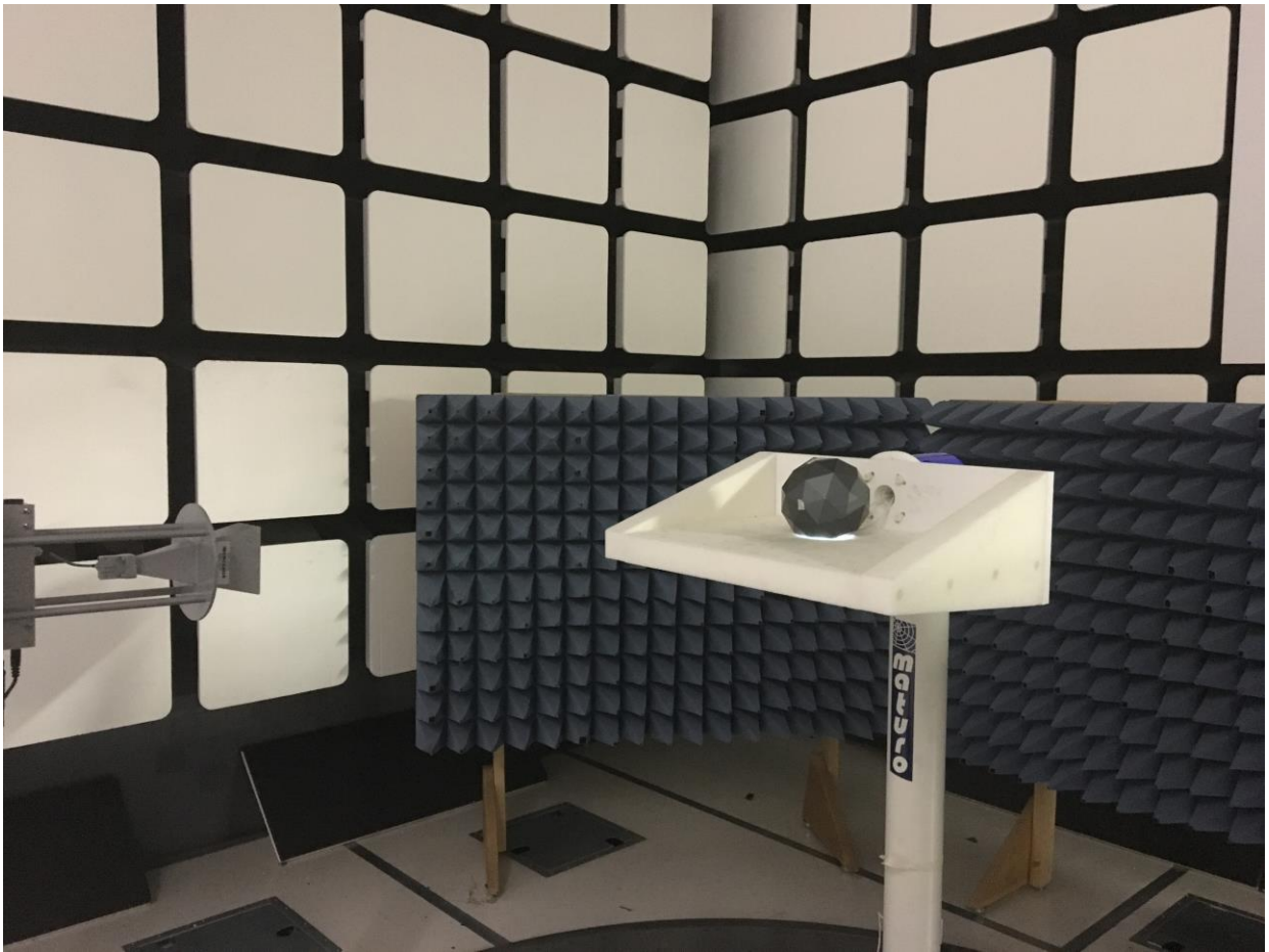
Figure 6: Test Setup for Radiated Emissions 18 GHz to 40 GHz (CDD and BT LE Modes)
