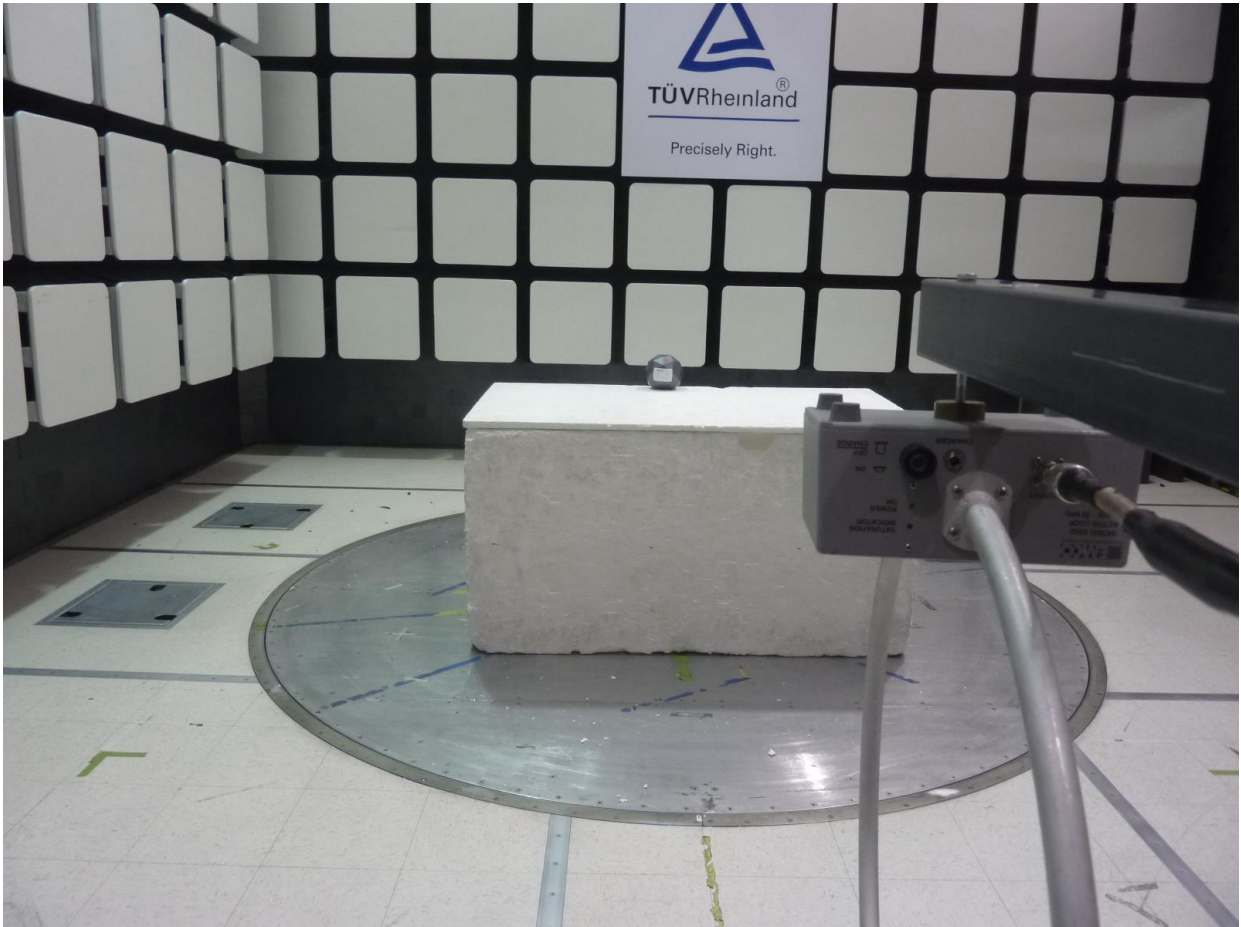
Figure 1: Test Setup for Radiated Emissions 9 kHz to 30 MHz (CDD and BT LE Modes)
