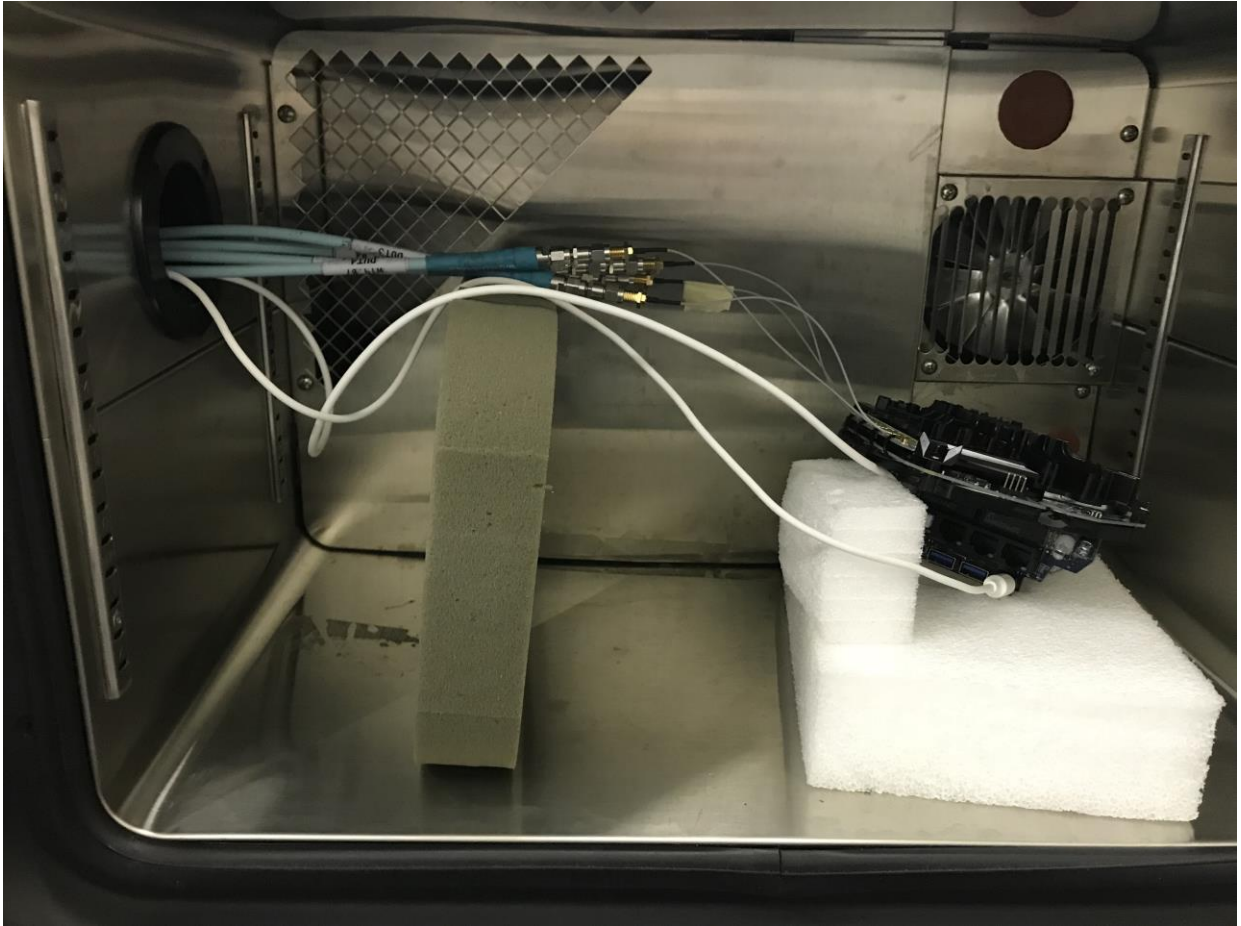
Figure 11: Test Setup for Conducted Emissions (Antenna Port- WLAN)
