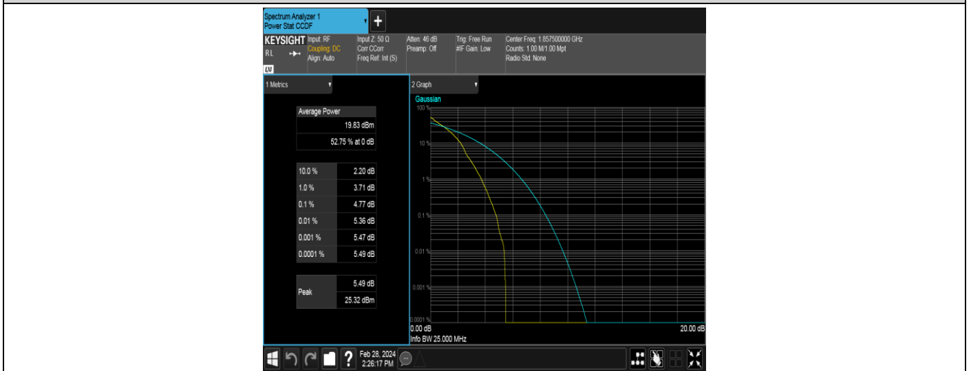
Band2-15MHz-QPSK-18675-75RB#0
