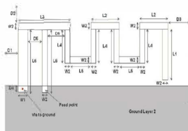
Figure 1: Antenna Dimensions
