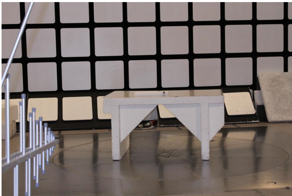
Photograph 2. Radiated emission 30 MHz to 1000 MHz.
