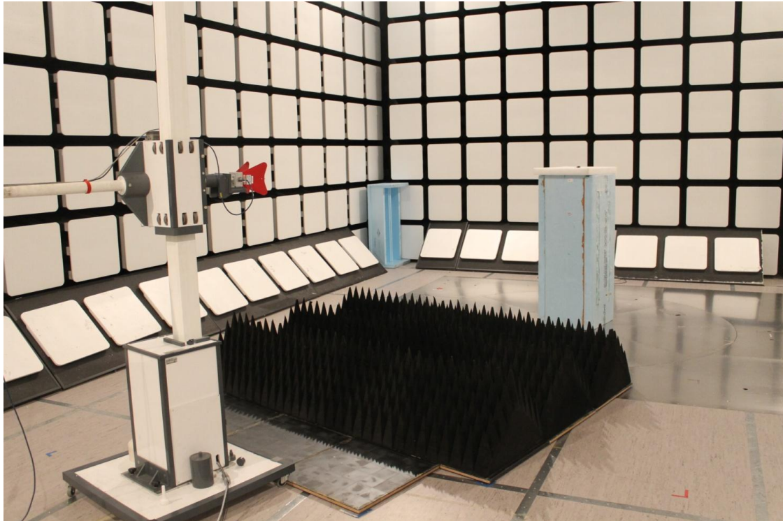
Photograph 3. Radiated emission 1 GHz to 18 GHz.
