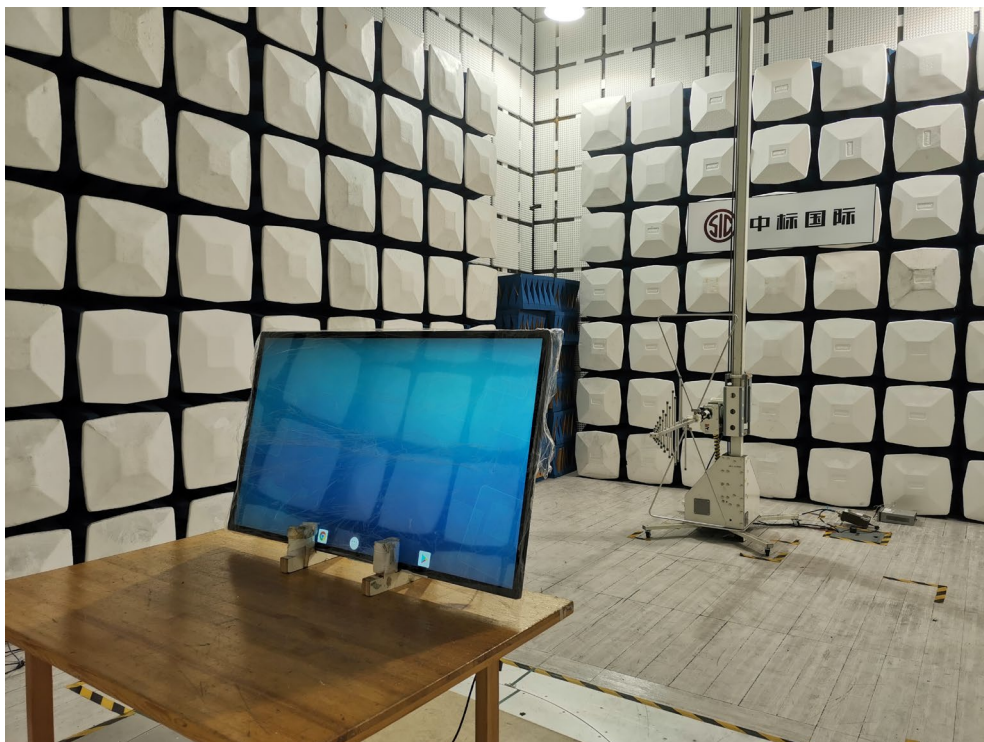
Radiated Spurious & Band Edge Emission (below 1GHz)
