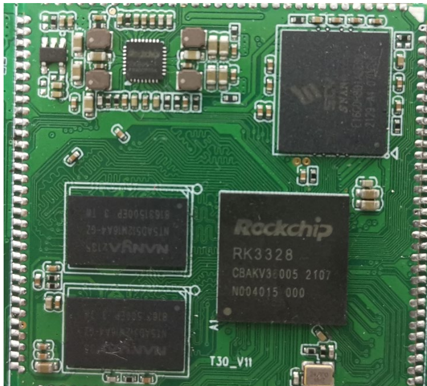
Mainboard Front 2
