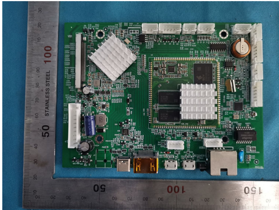
Mainboard Front 1
