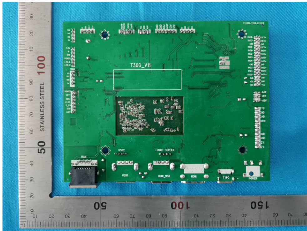
Mainboard Back
