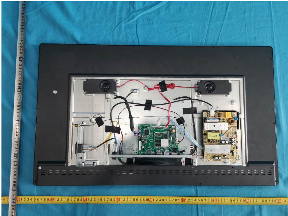
Internal Structure 2
