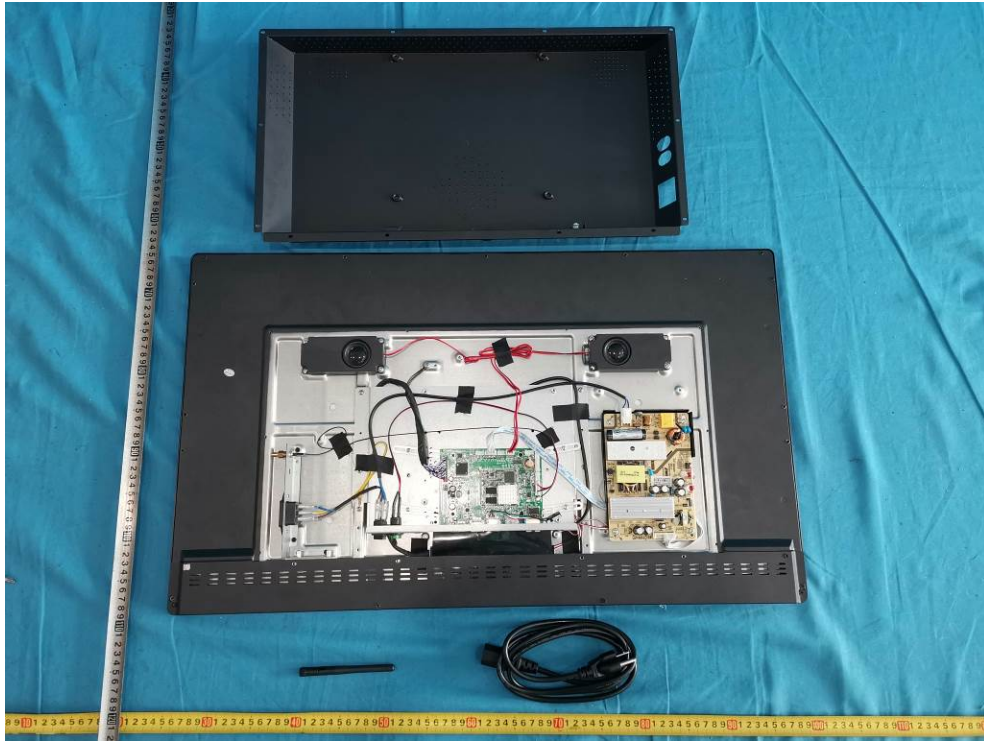
Internal Structure 1
