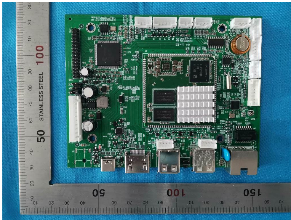
Mainboard Front 1
