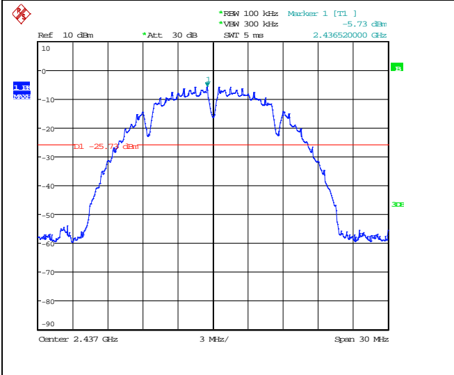
Channel 6 / 2437 MHz
